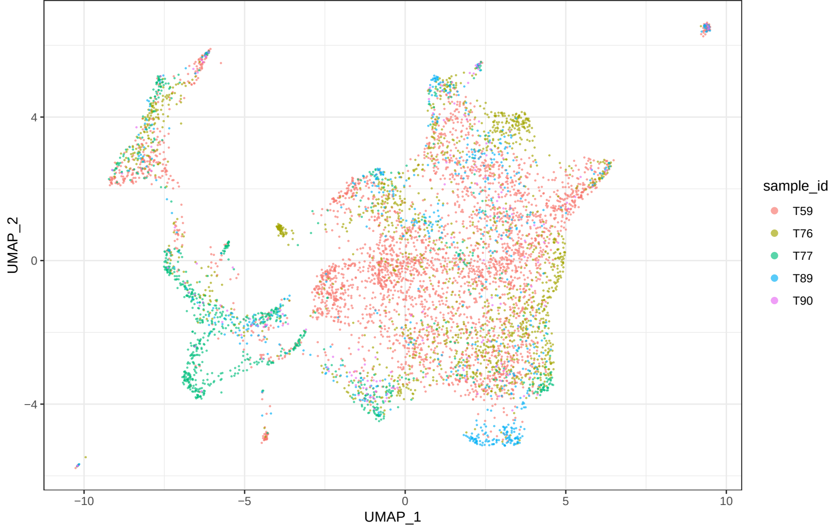
GSE154600 Myeloid_like C_RPCA samples
