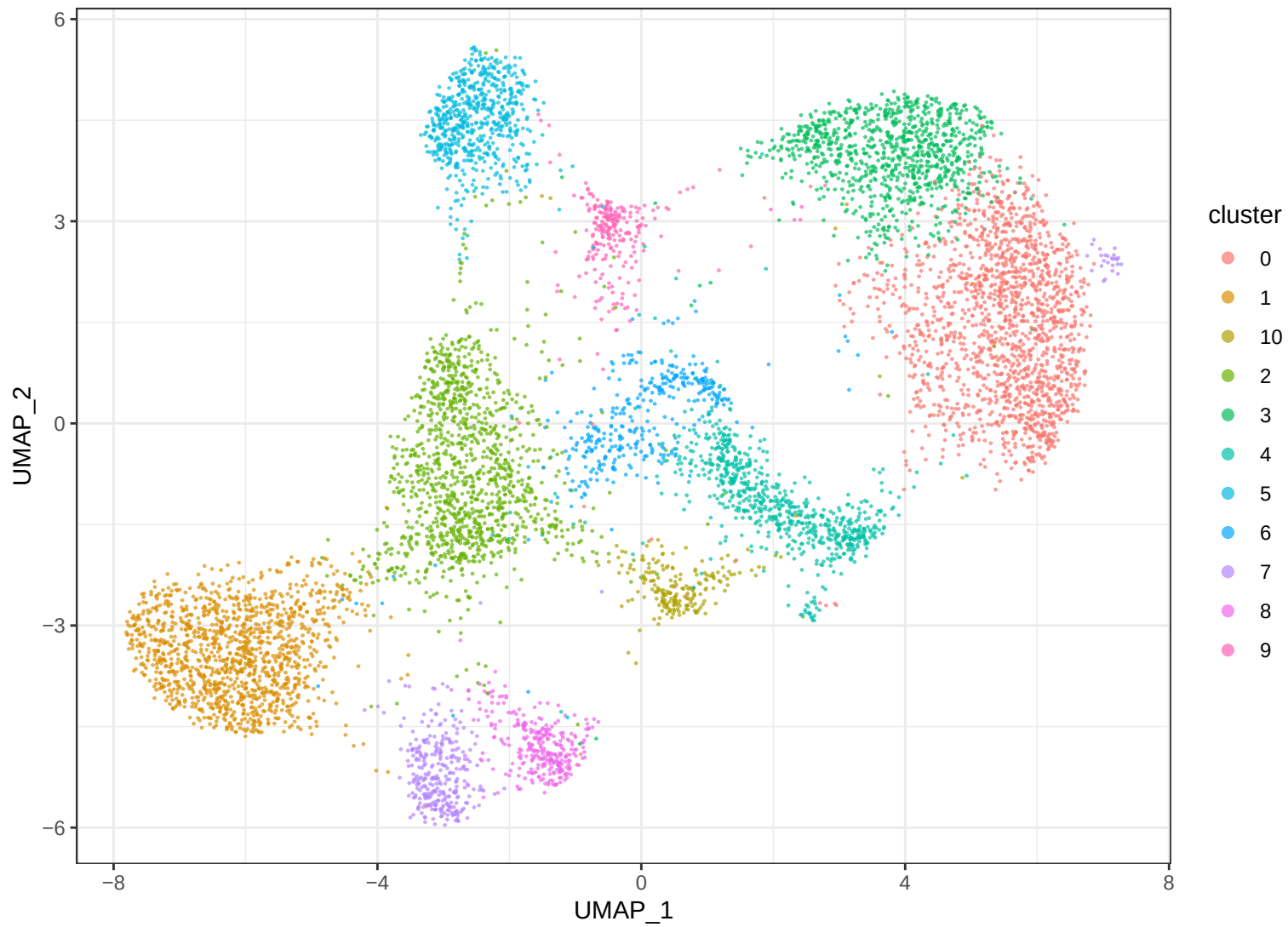
GSE154600 T_NK_like B_harmony_sample clusters
