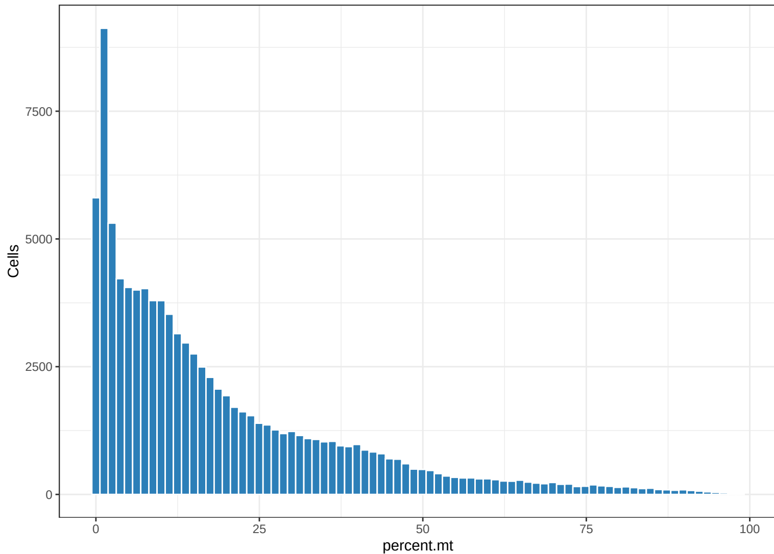
GSE158722 repaired percent.mt
