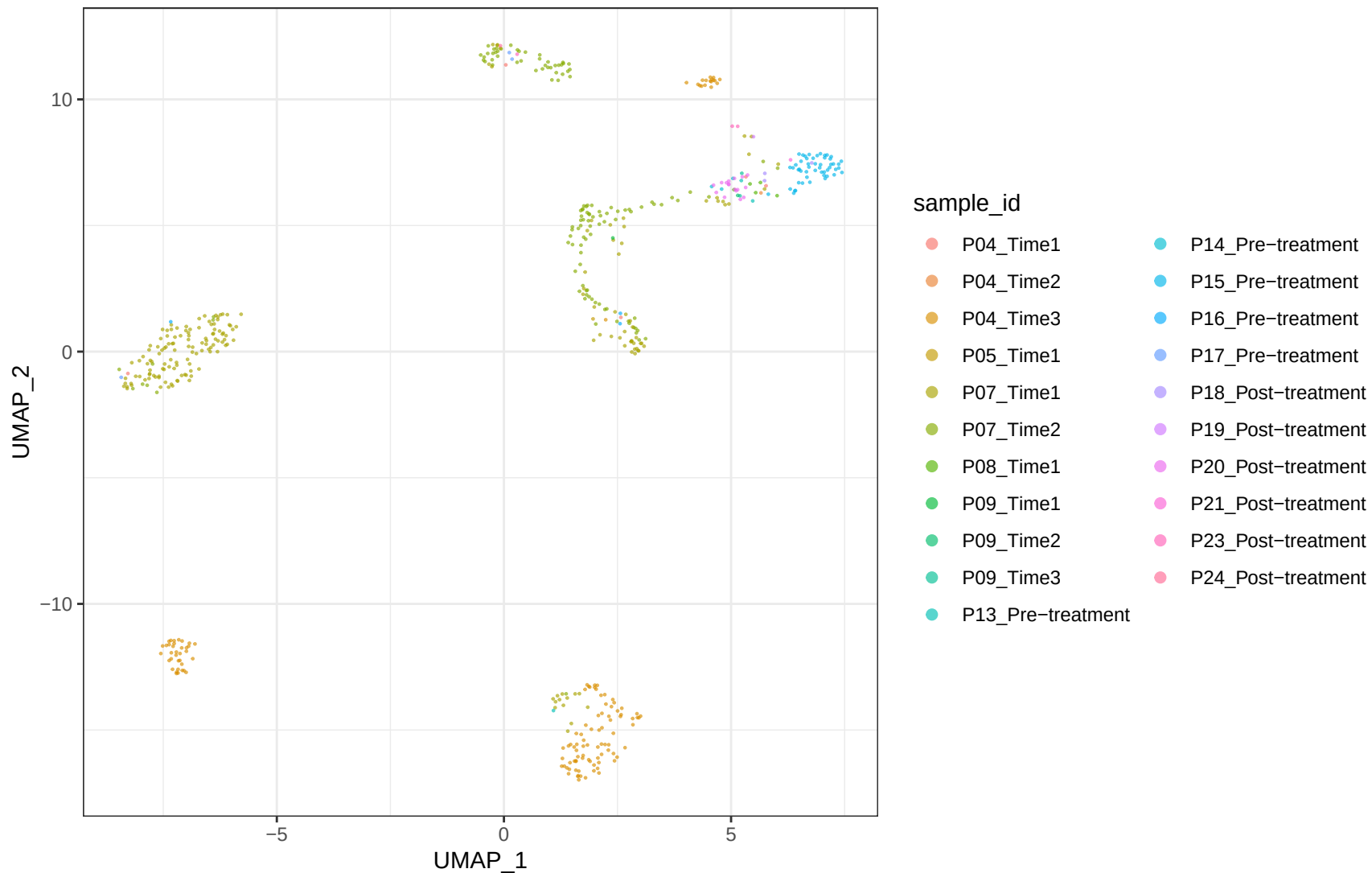
GSE158722 B_Plasma_like A_uncorrected samples
