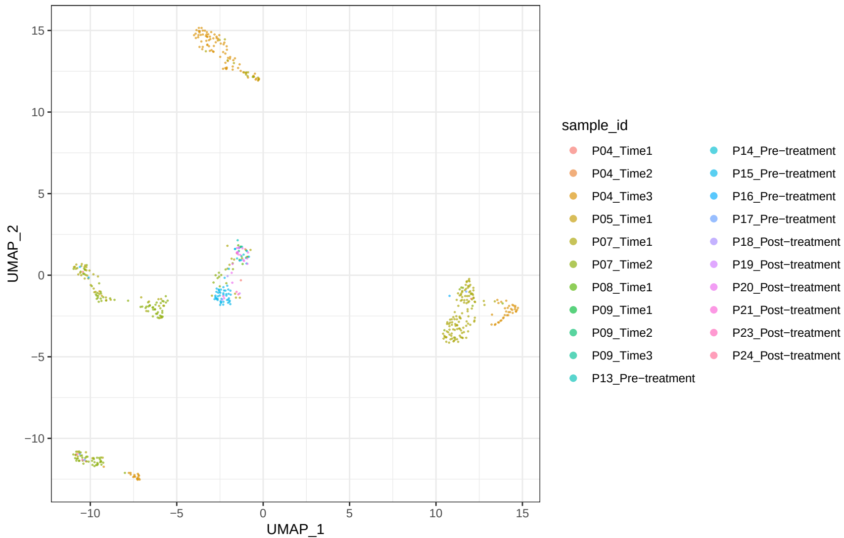
GSE158722 B_Plasma_like B_harmony_sample samples
