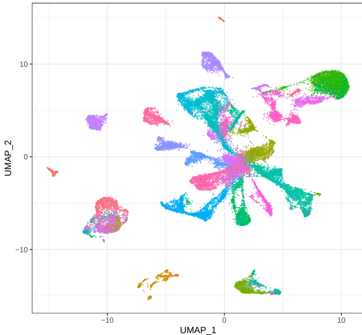
GSE158722 Combined_broad_lineages A_uncorrected samples
