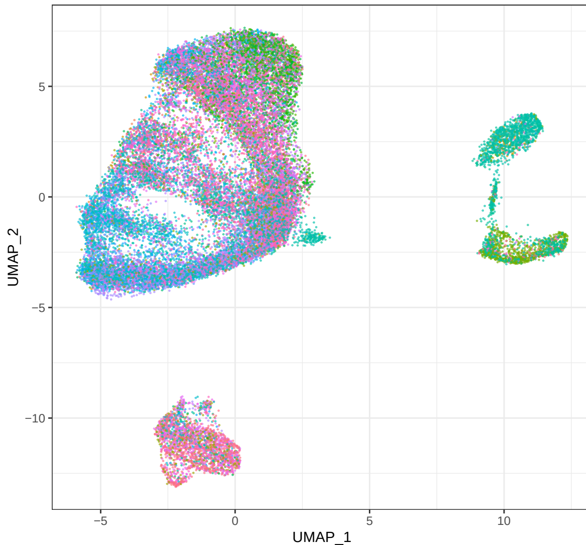
GSE158722 Combined_broad_lineages B_harmony_sample samples
