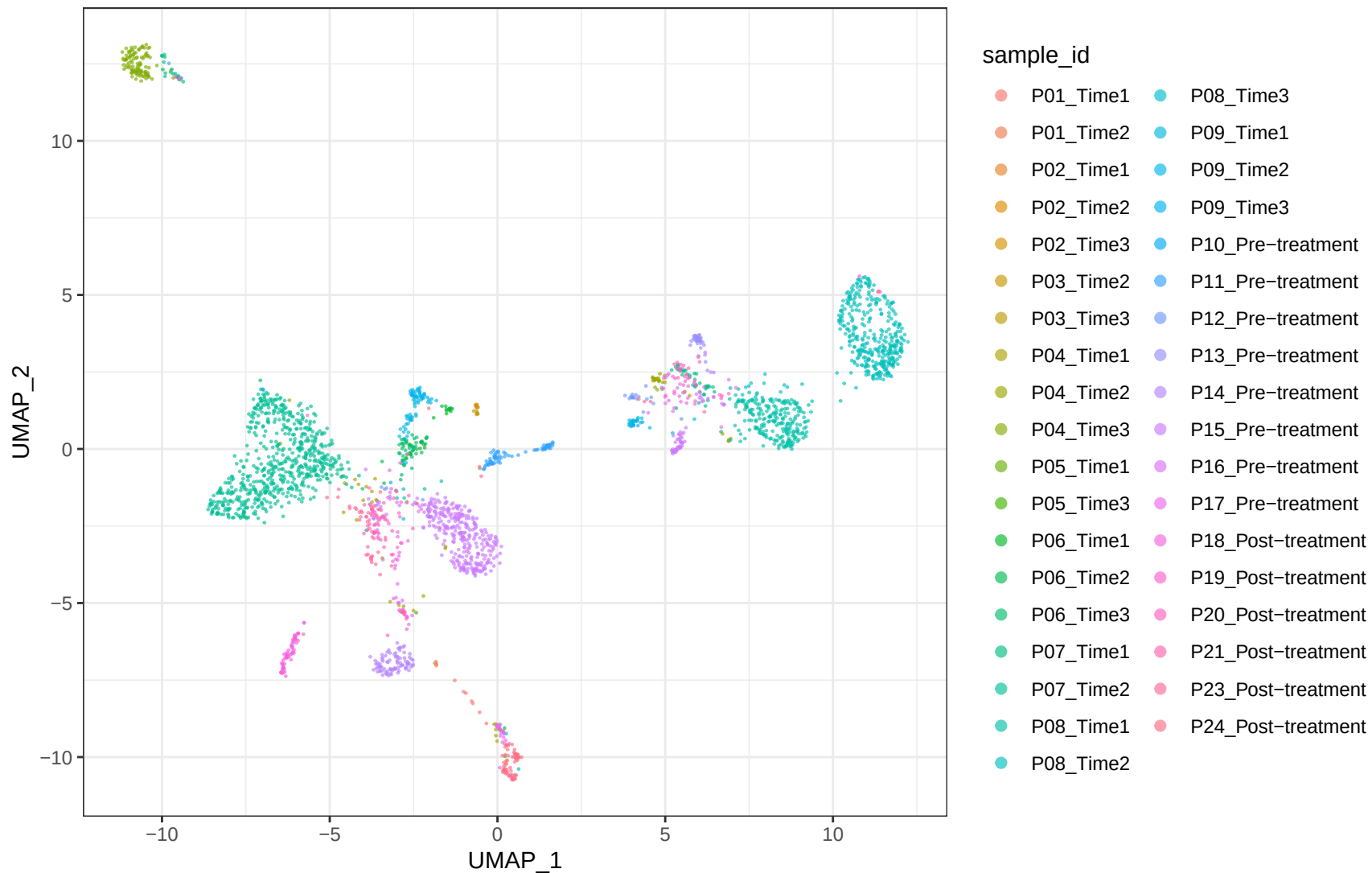
GSE158722 Cycling_like A_uncorrected samples
