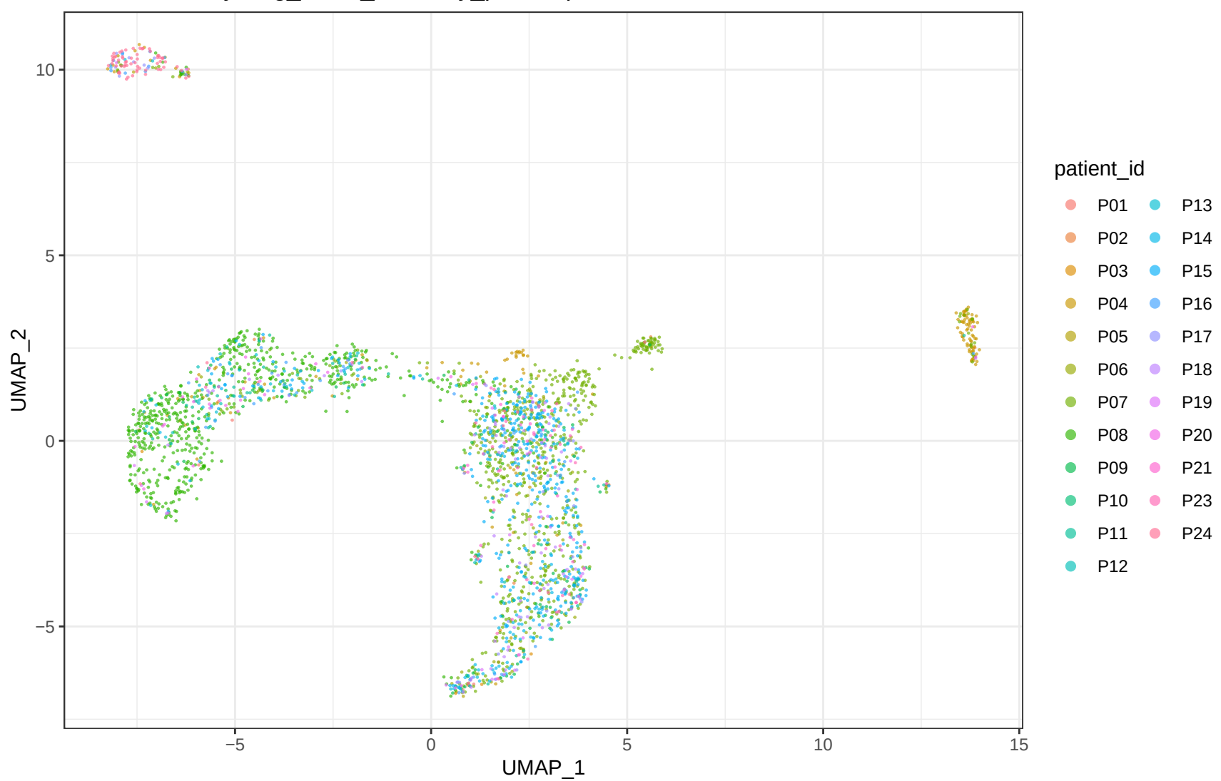
GSE158722 Cycling_like B_harmony_patient patients
