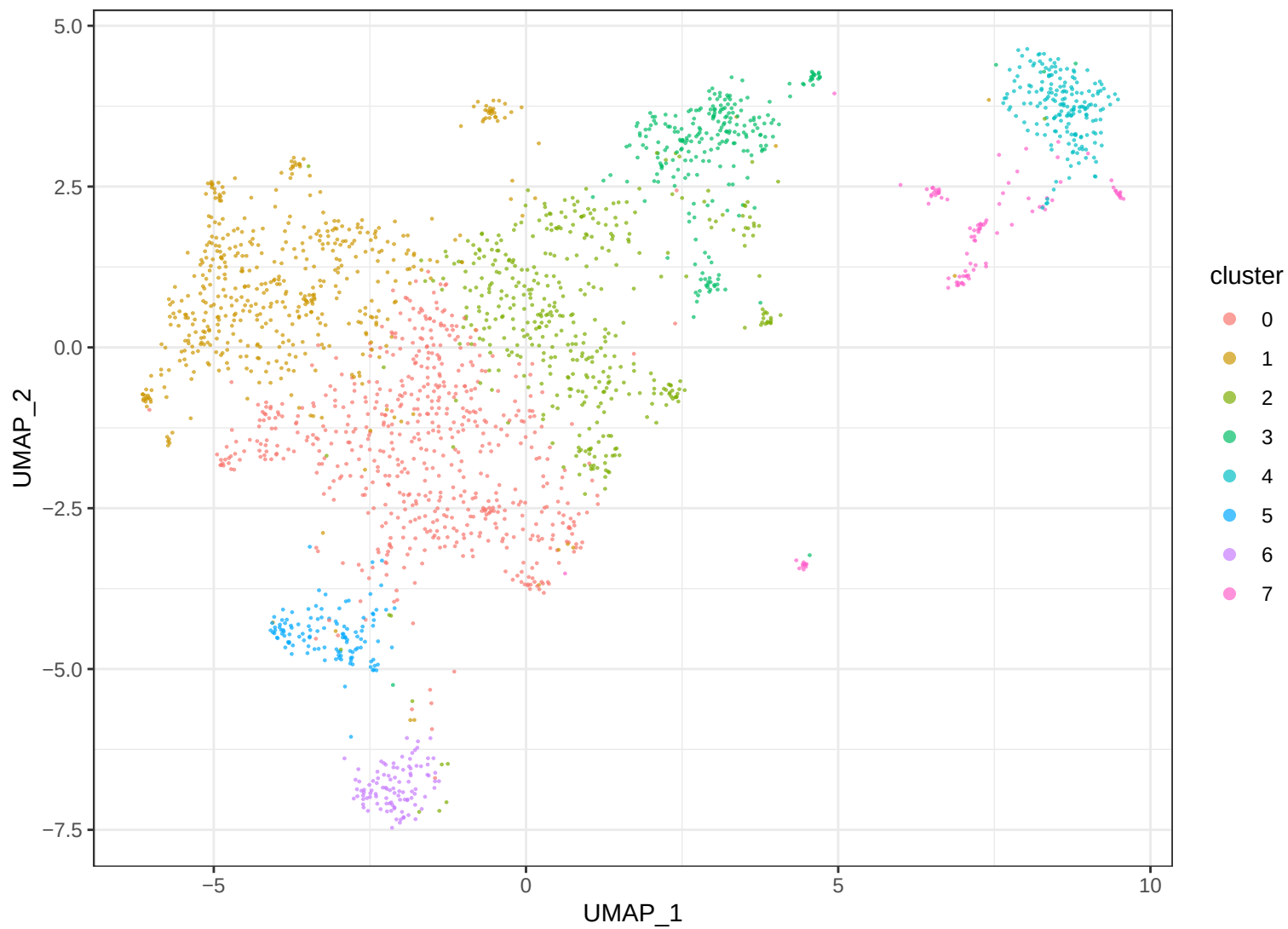
GSE158722 Fibroblast_like B_harmony_sample clusters
