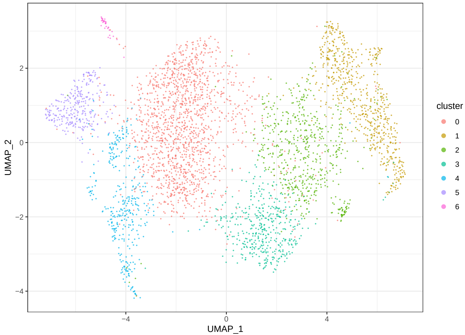
GSE158722 Myeloid_like B_harmony_patient clusters
