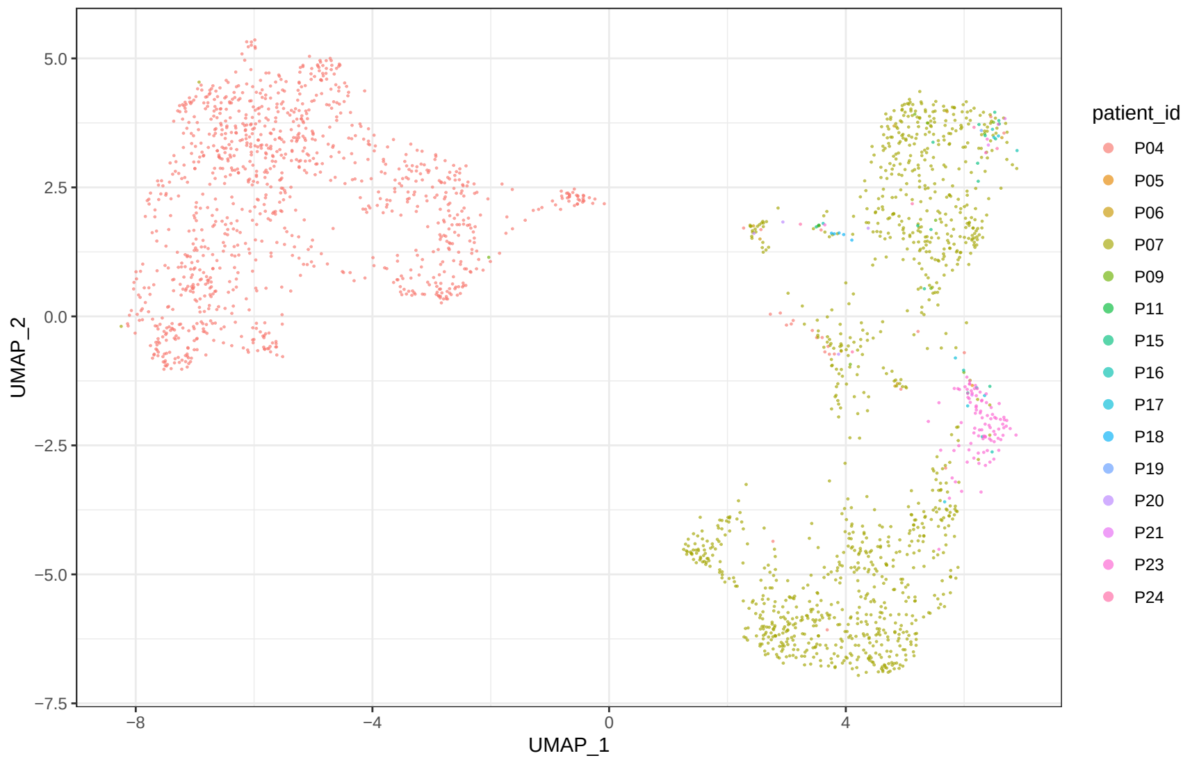
GSE158722 T_NK_like B_harmony_patient patients
