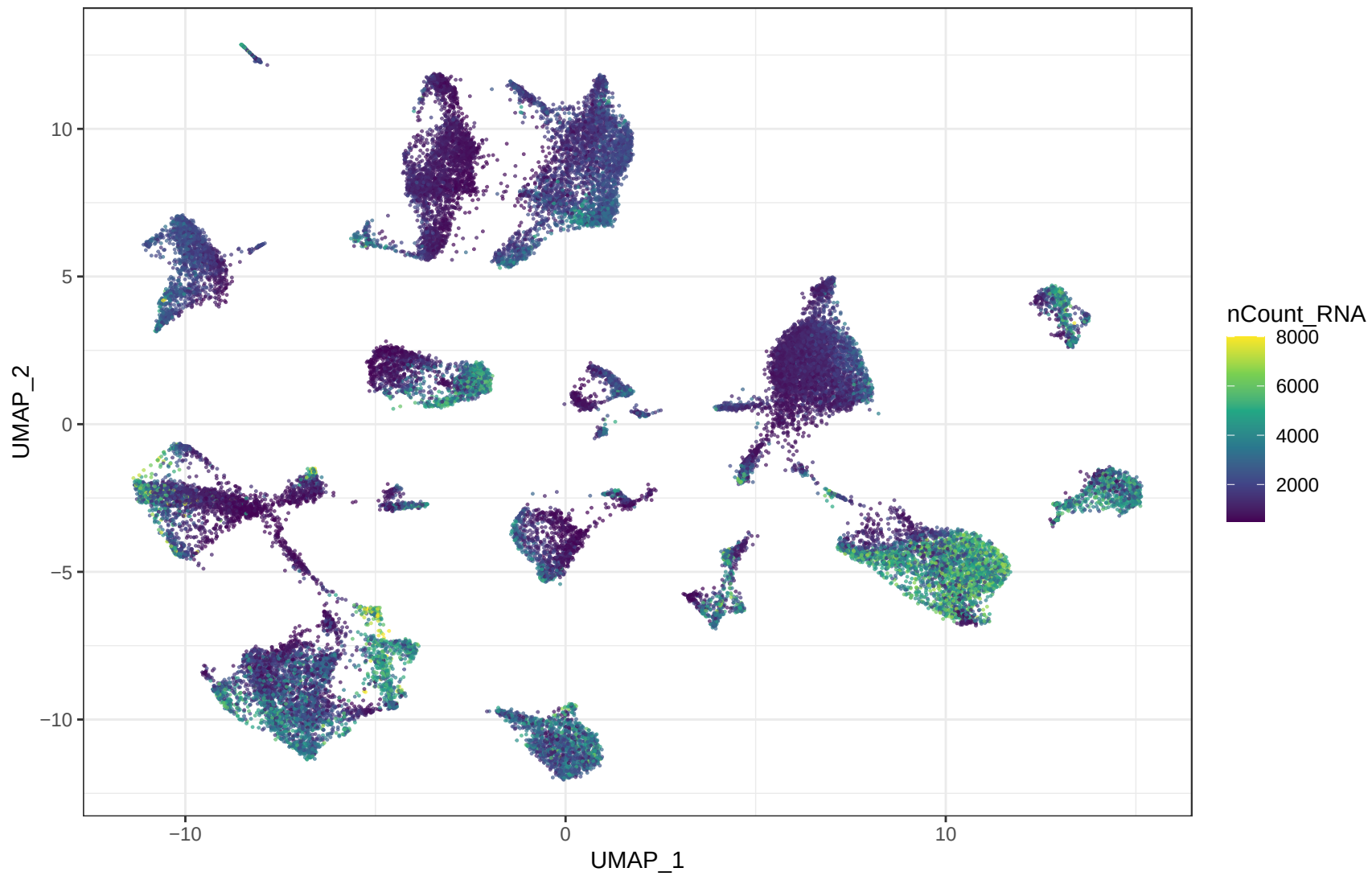
GSE154600 UMAP_by_nCount
