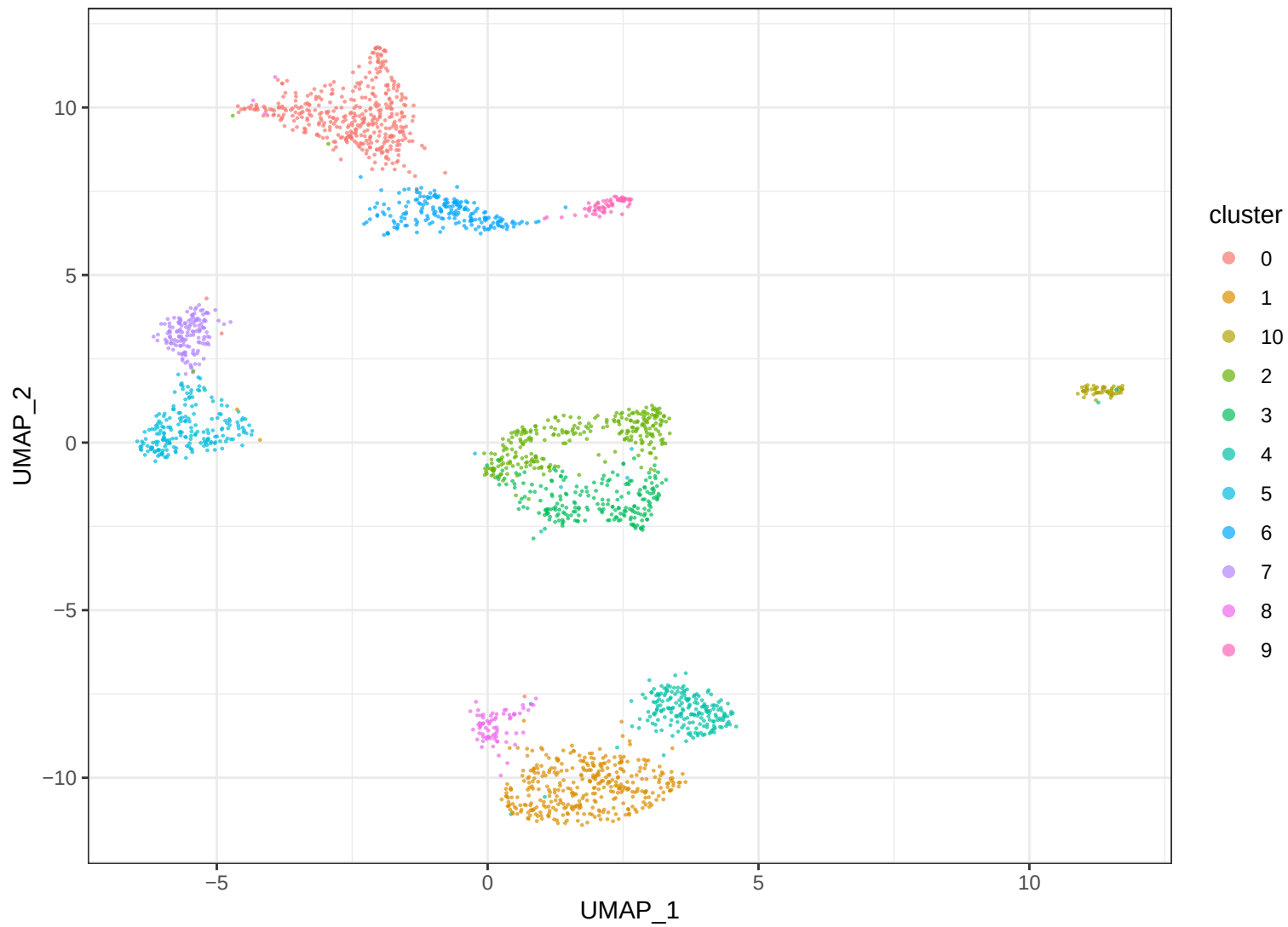
GSE154600 B_Plasma_like A_uncorrected clusters
