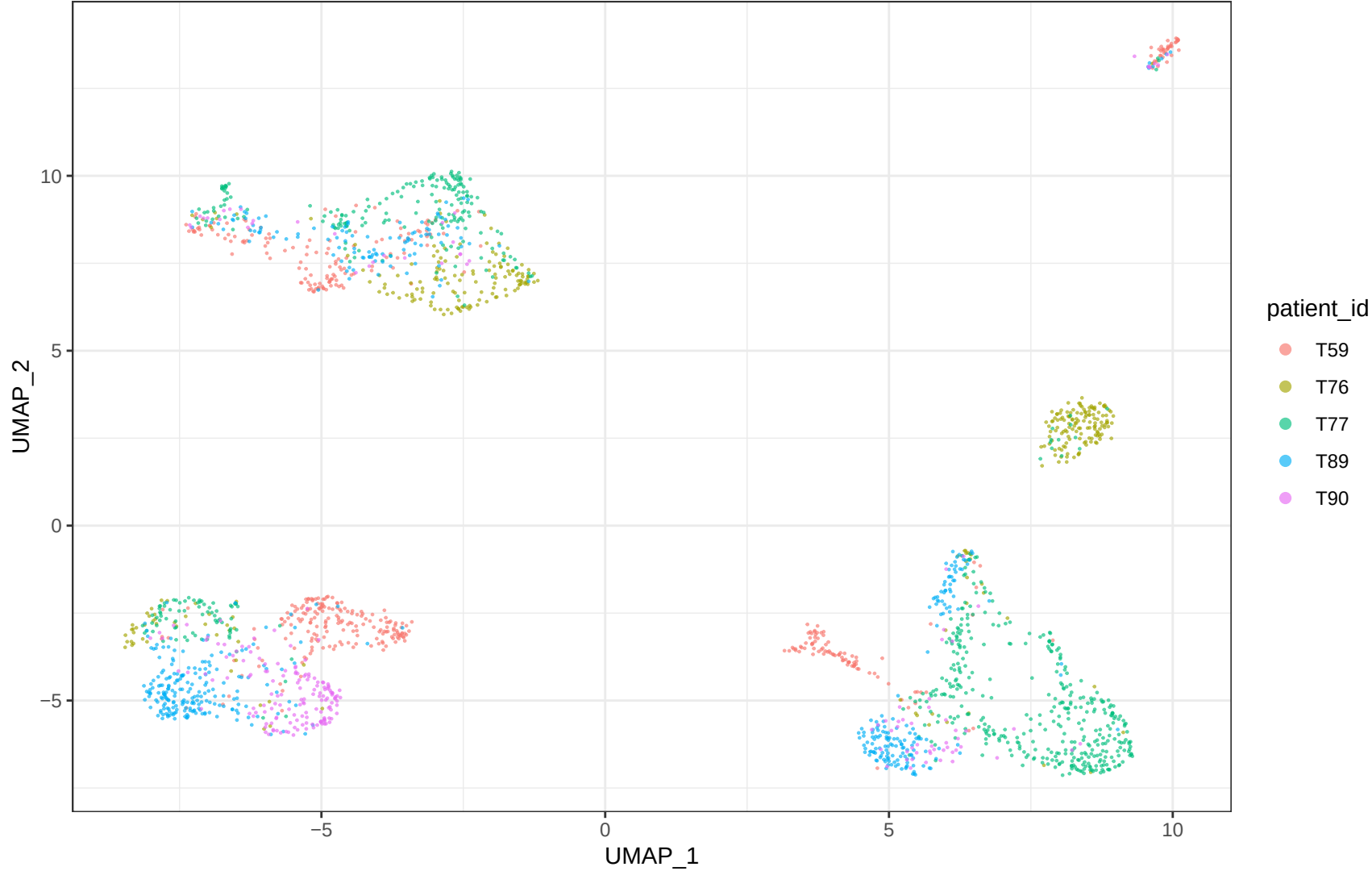
GSE154600 B_Plasma_like C_RPCA patients
