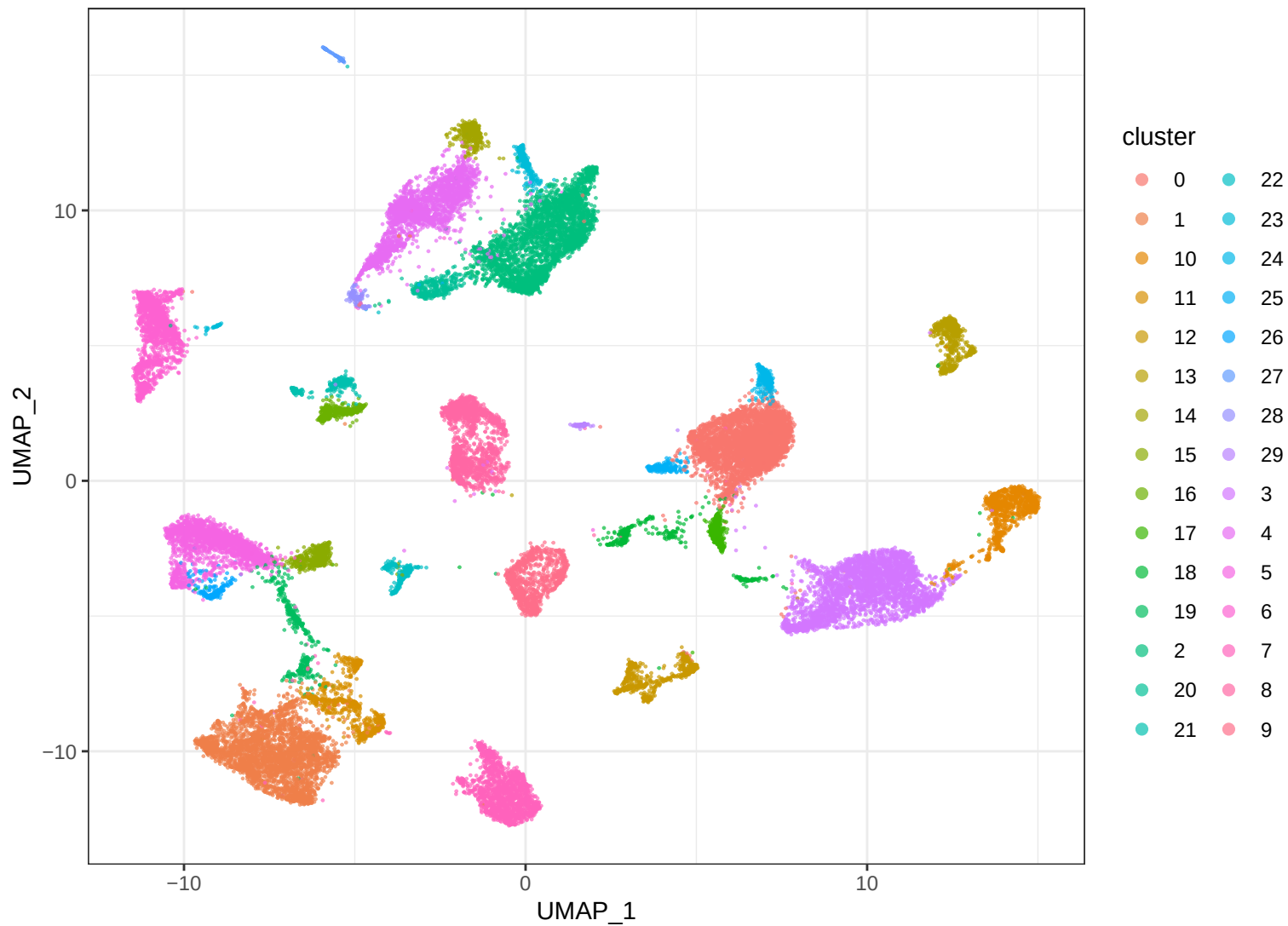
GSE154600 Combined_broad_lineages A_uncorrected clusters
