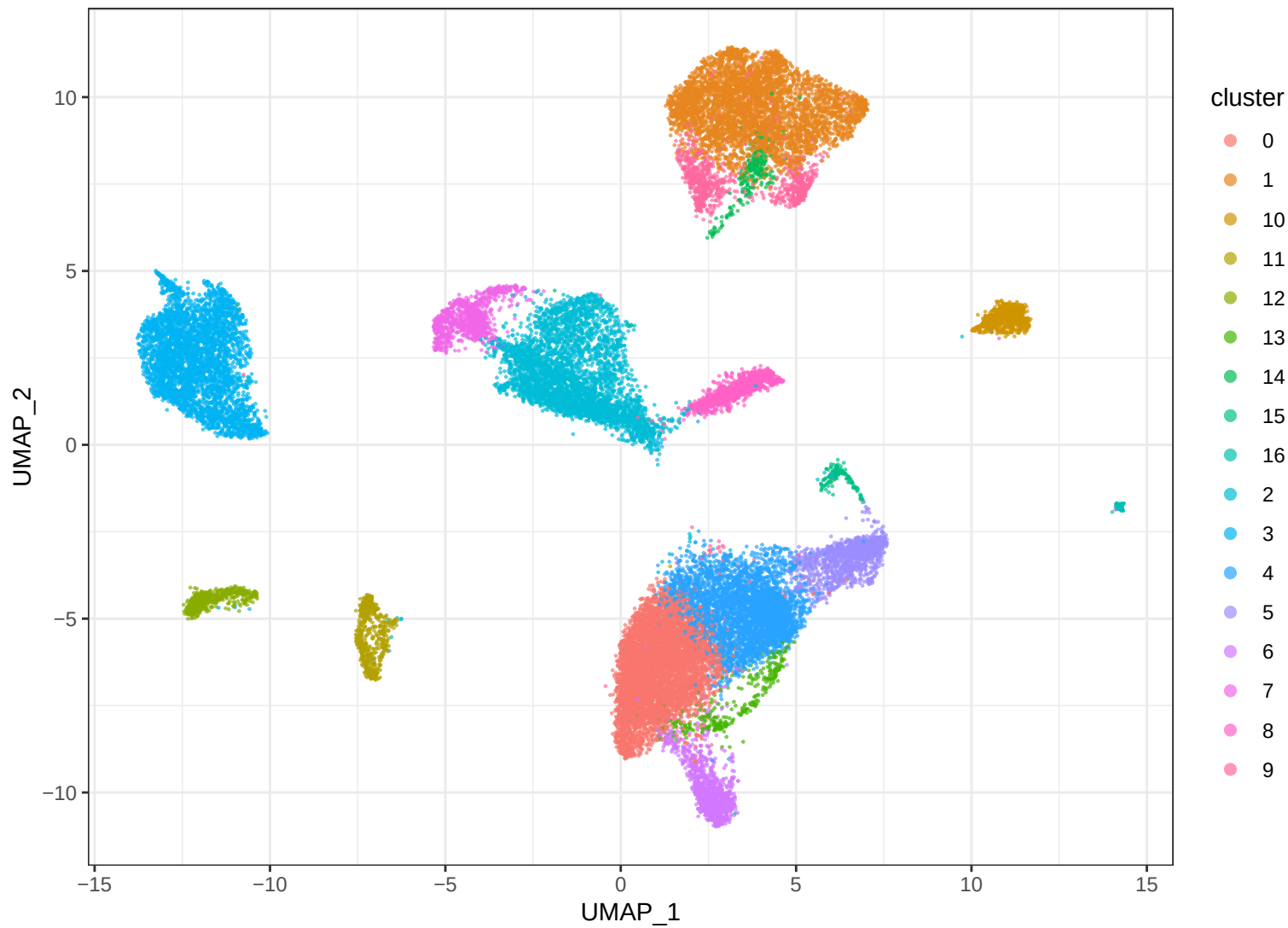
GSE154600 Combined_broad_lineages B_harmony_sample clusters
