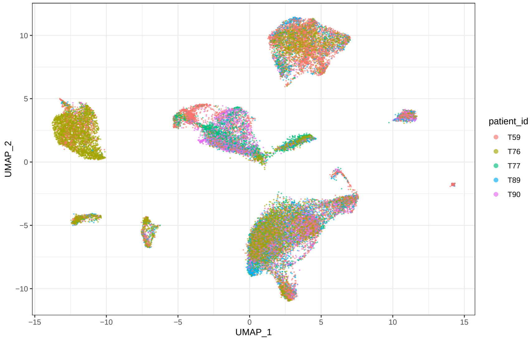
GSE154600 Combined_broad_lineages B_harmony_sample patients
