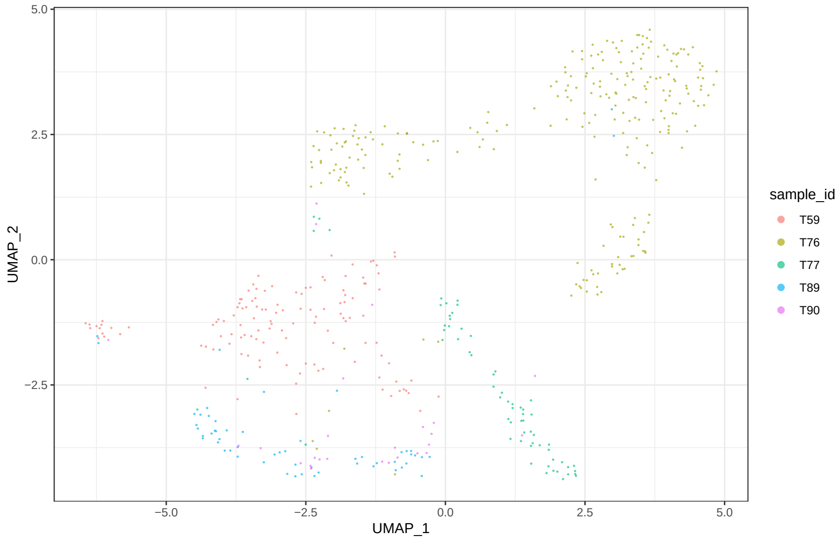
GSE154600 Endothelial_like A_uncorrected samples
