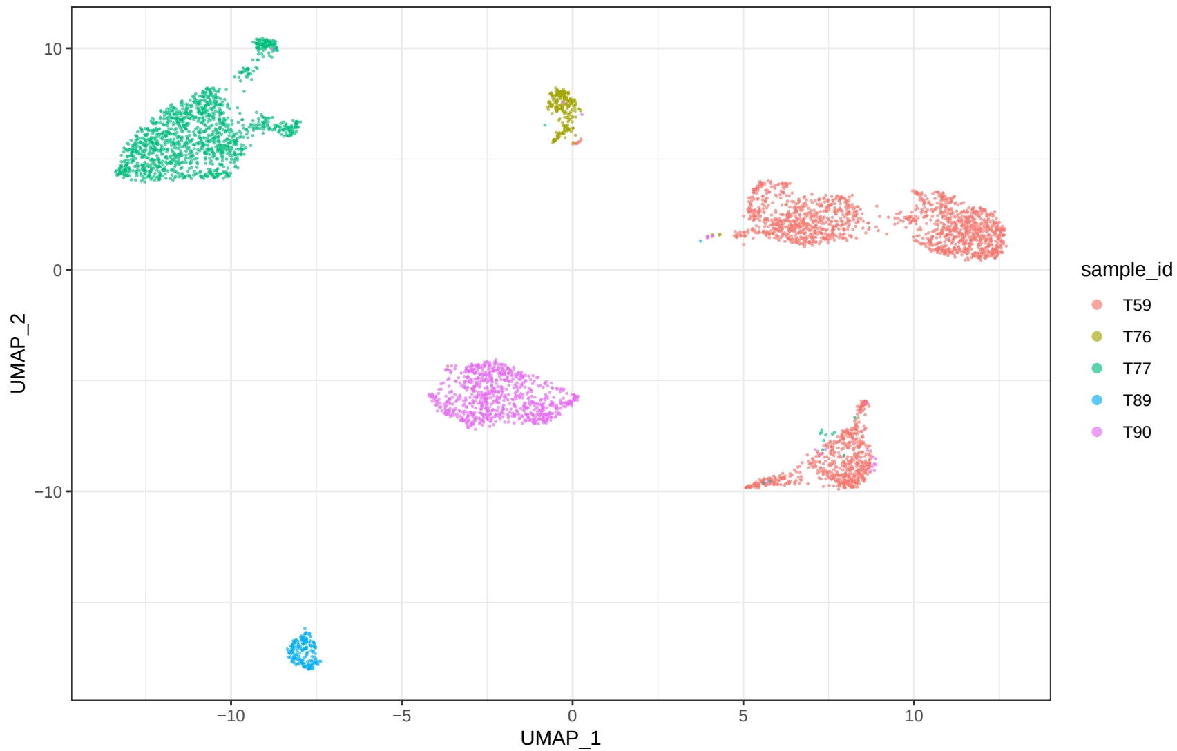
GSE154600 Epithelial_like A_uncorrected samples
