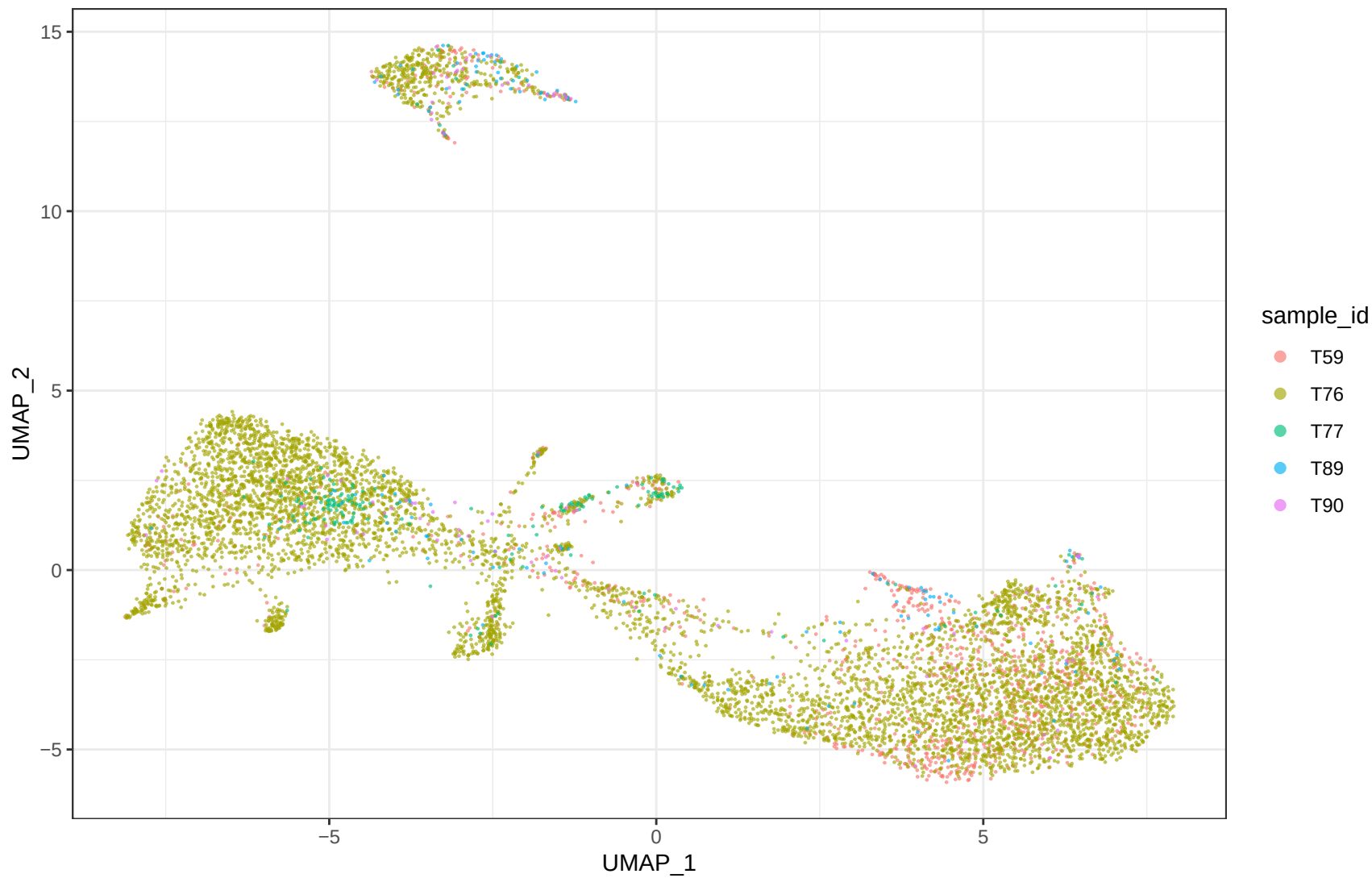
GSE154600 Fibroblast_like B_harmony_sample samples
