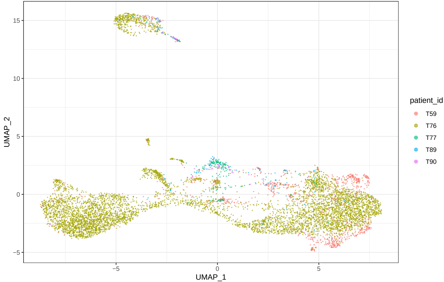
GSE154600 Fibroblast_like C_RPCA patients
