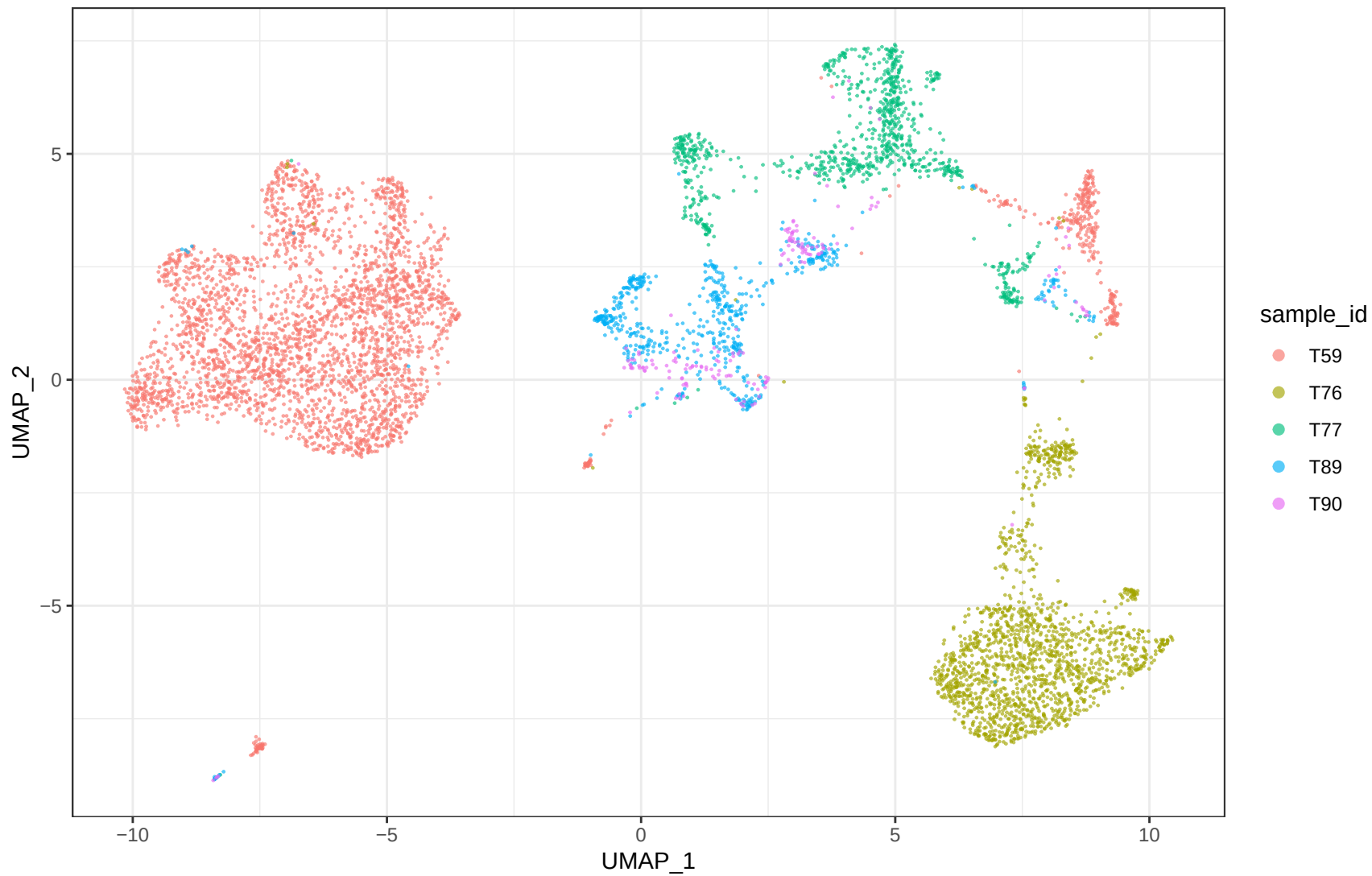
GSE154600 Myeloid_like A_uncorrected samples
