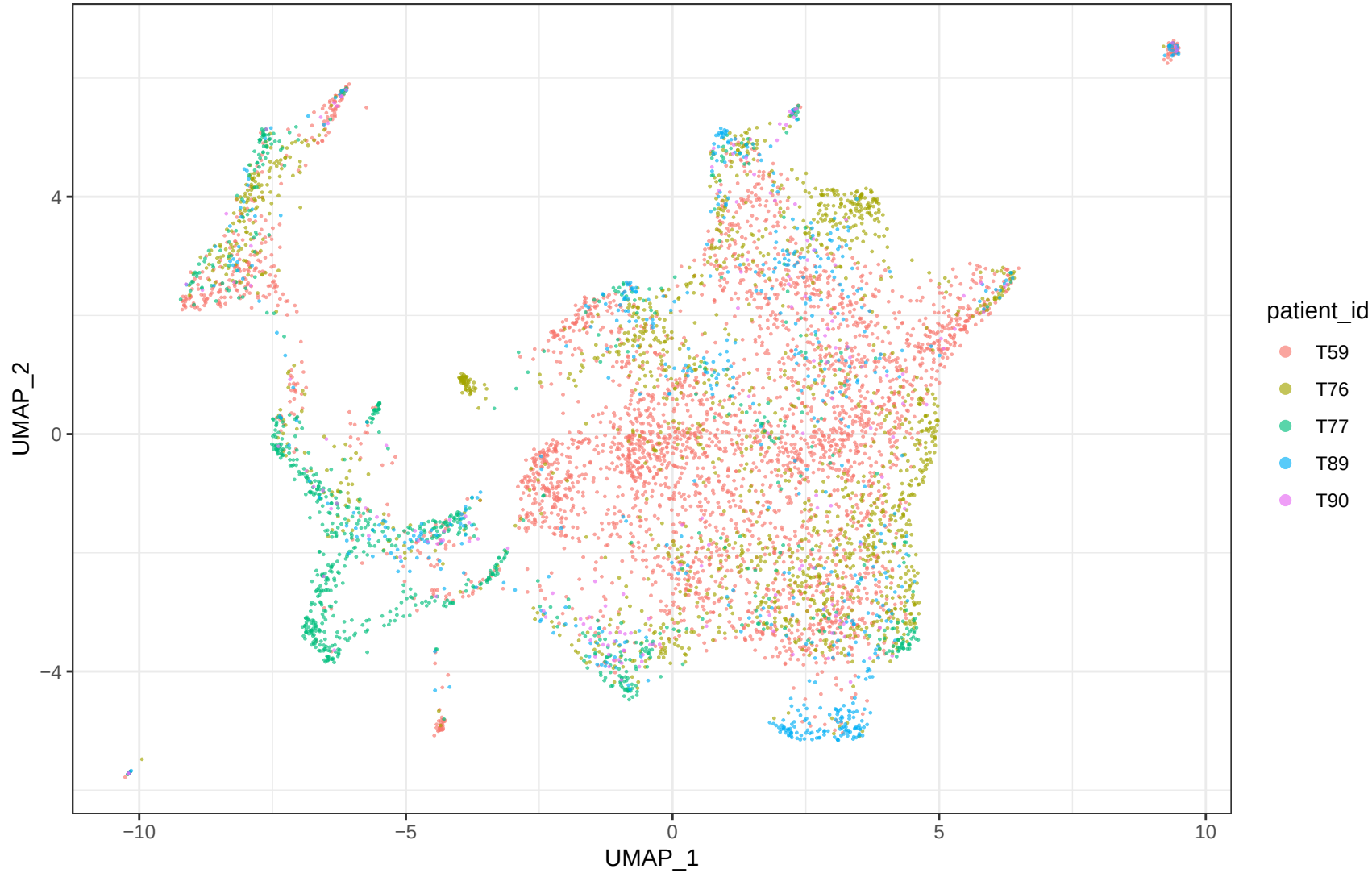
GSE154600 Myeloid_like C_RPCA patients
