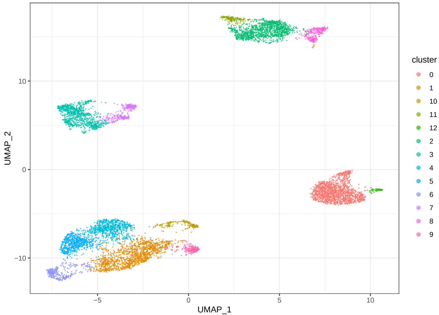
GSE154600 T_NK_like A_uncorrected clusters
