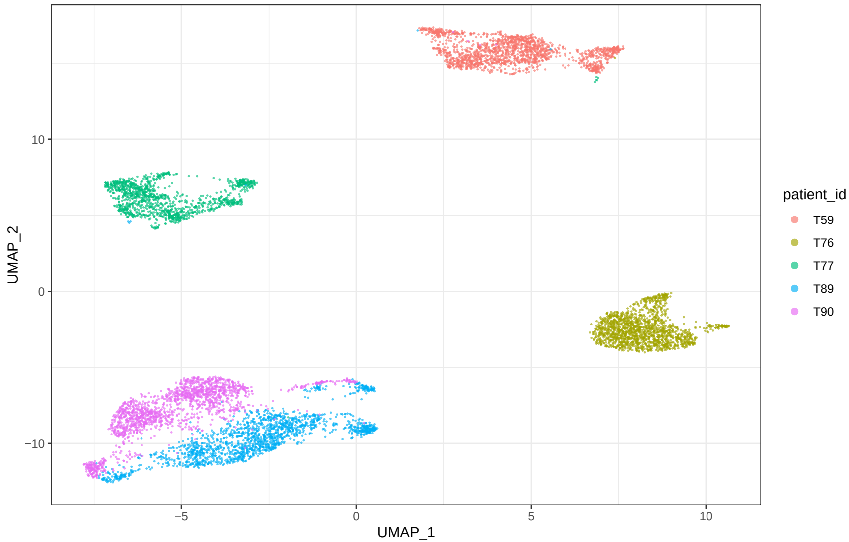
GSE154600 T_NK_like A_uncorrected patients
