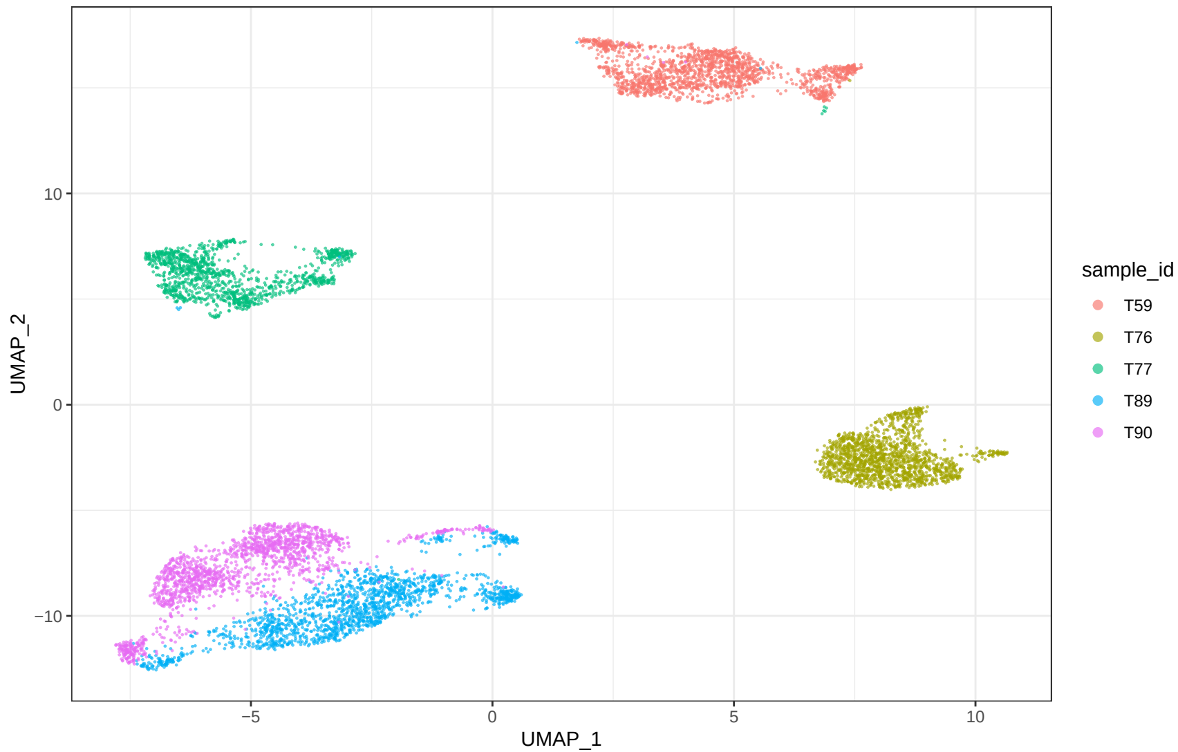
GSE154600 T_NK_like A_uncorrected samples
