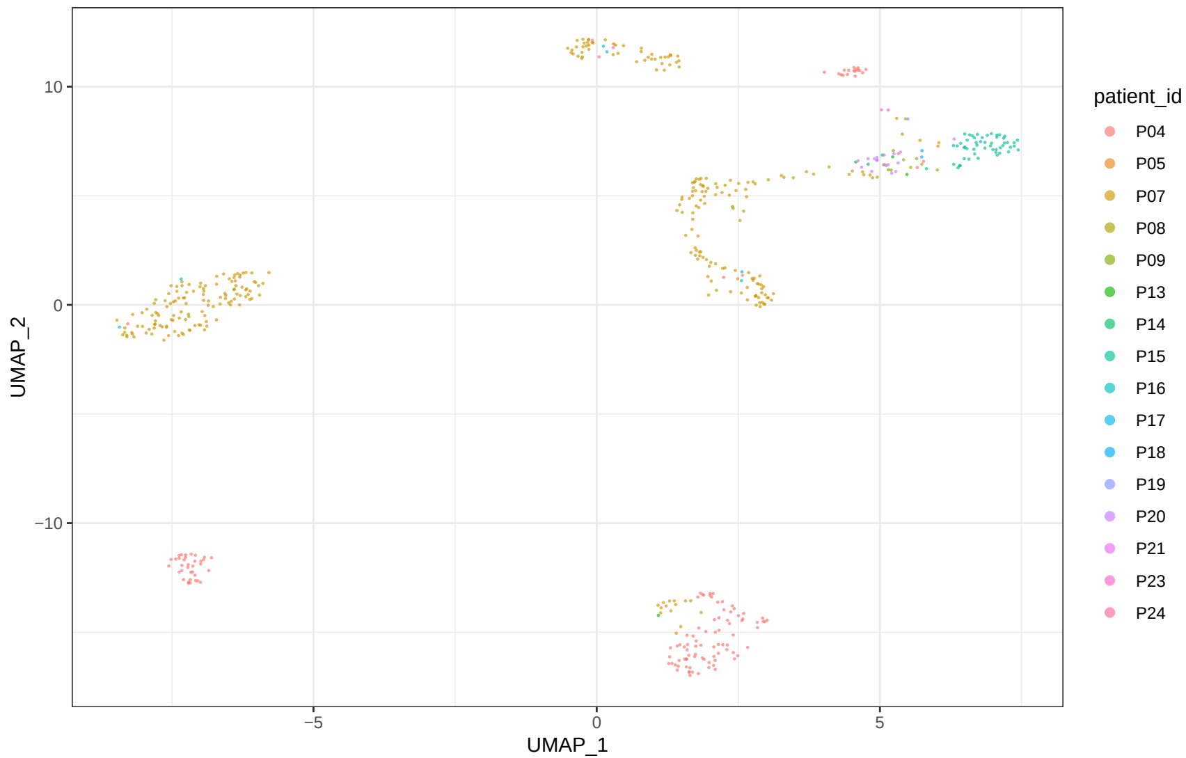
GSE158722 B_Plasma_like A_uncorrected patients
