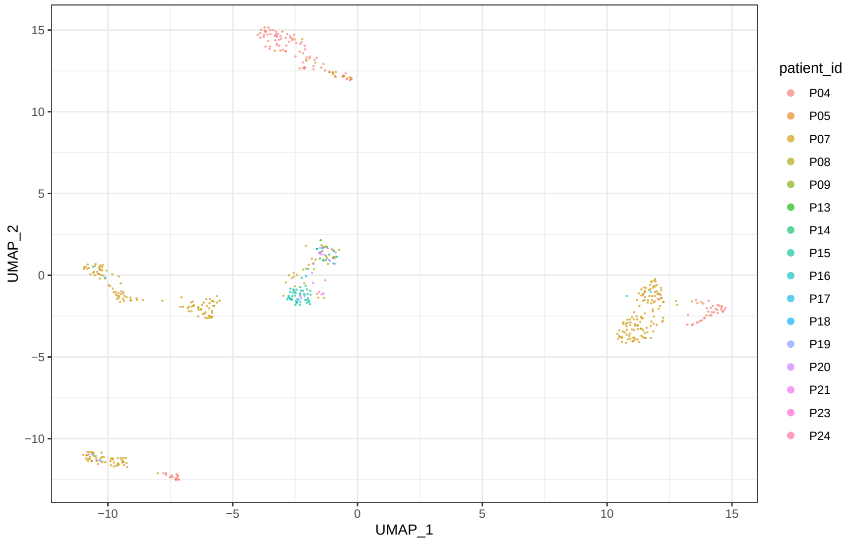
GSE158722 B_Plasma_like B_harmony_sample patients
