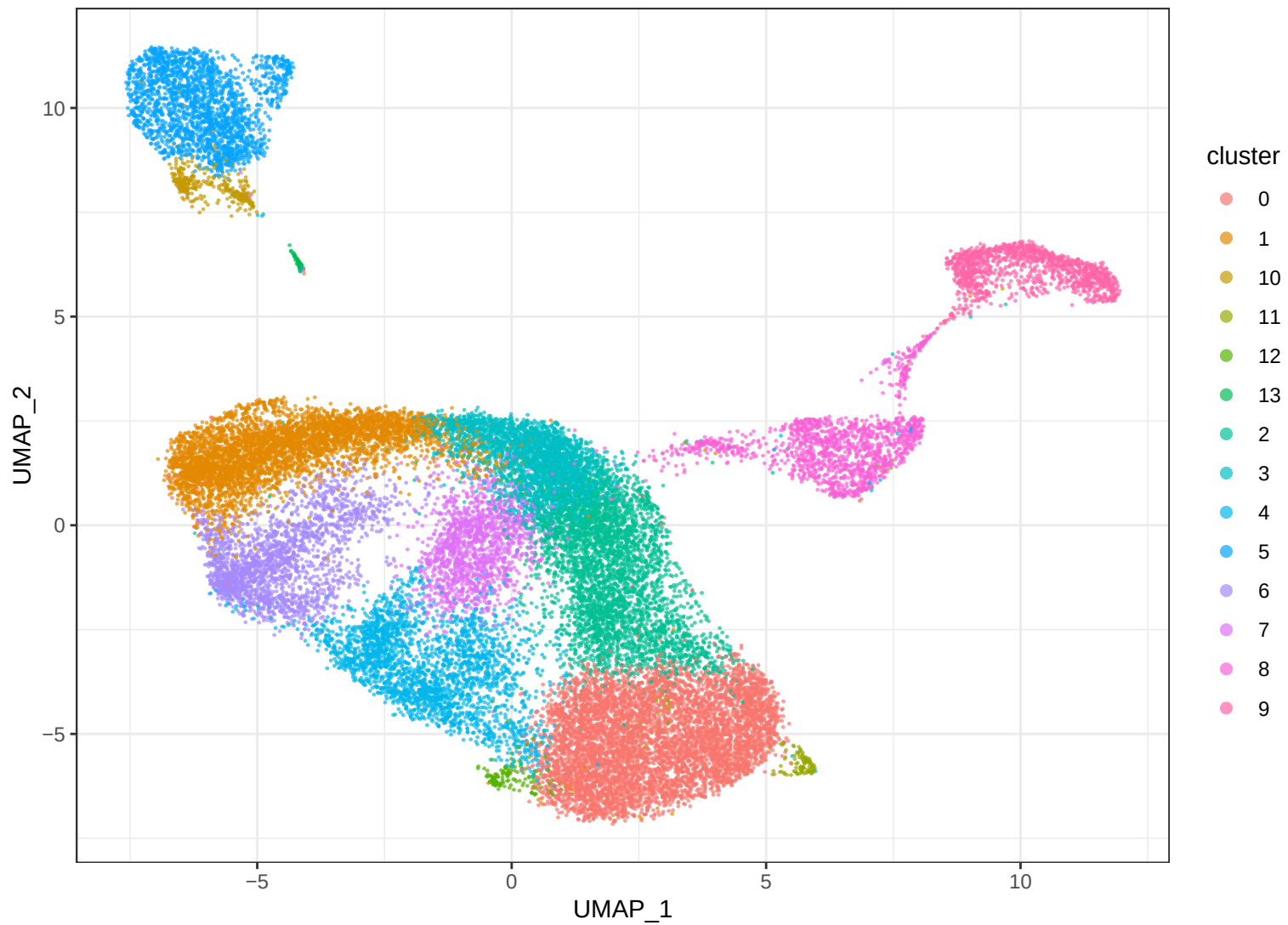
GSE158722 Combined_broad_lineages B_harmony_patient clusters
