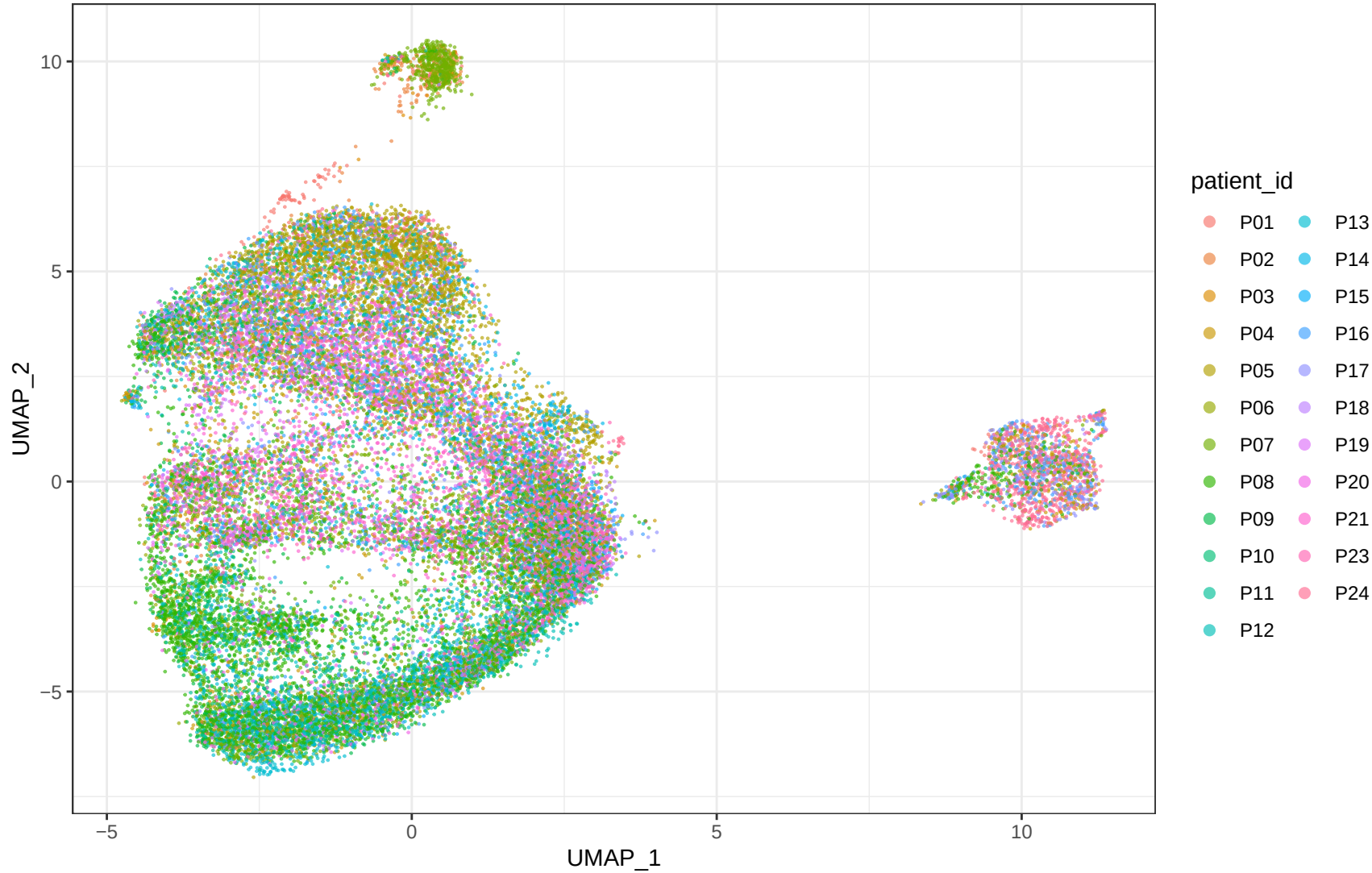
GSE158722 Epithelial_like B_harmony_sample patients
