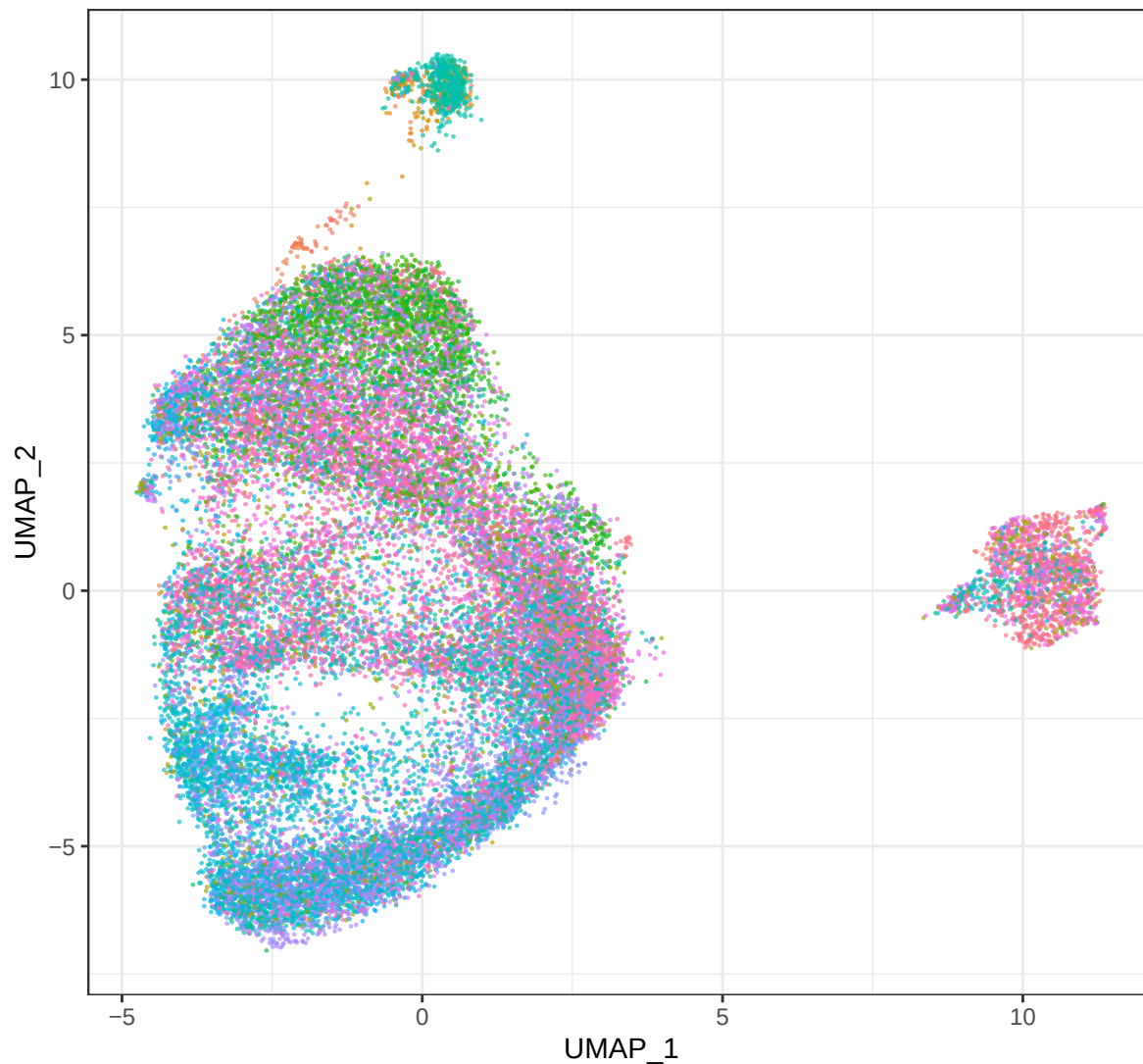
GSE158722 Epithelial_like B_harmony_sample samples
