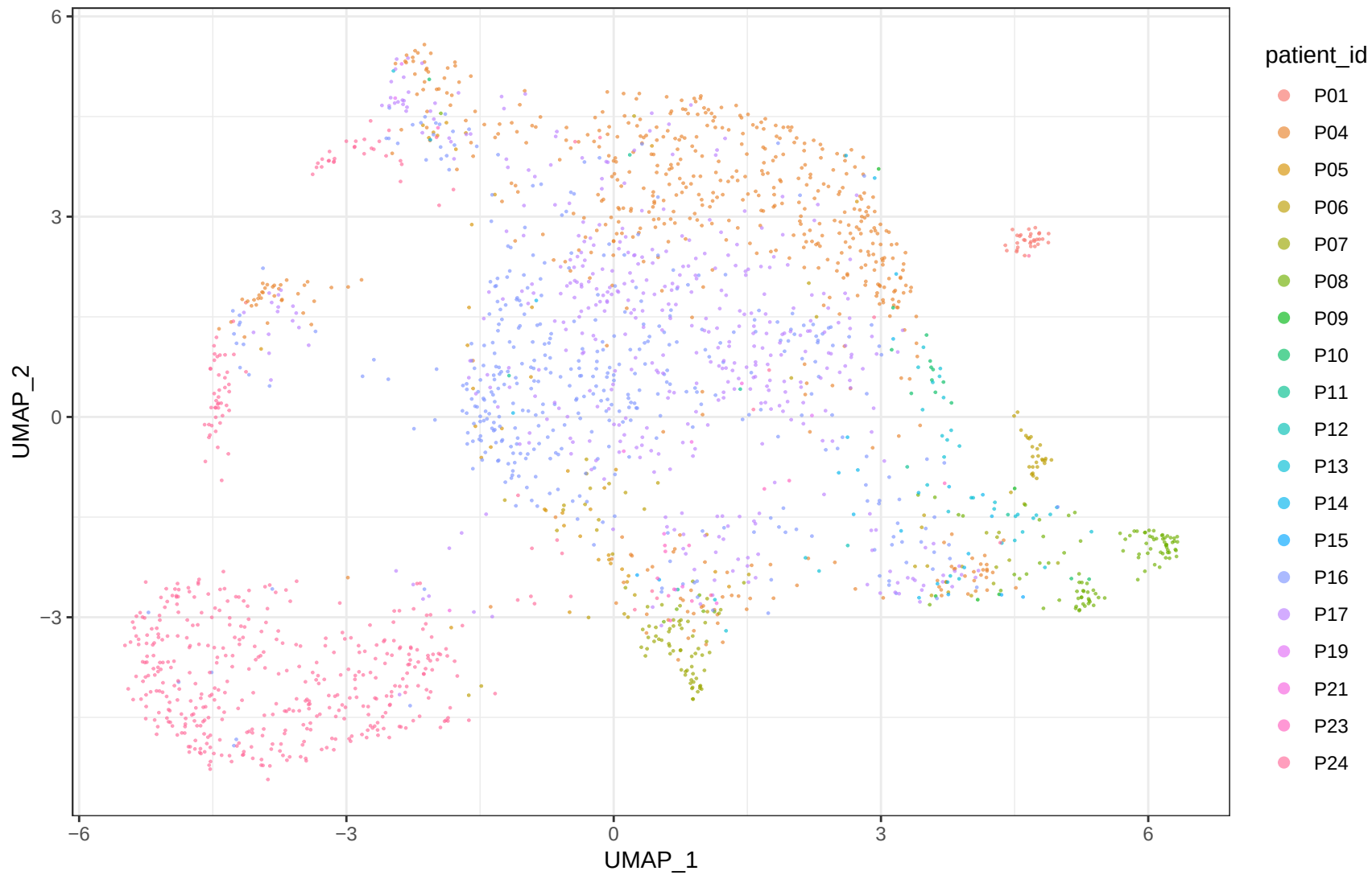
GSE158722 Fibroblast_like A_uncorrected patients
