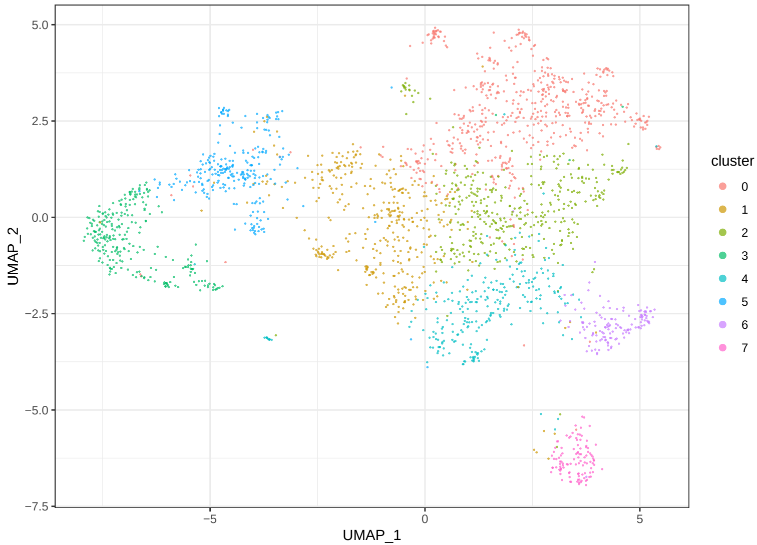
GSE158722 Fibroblast_like B_harmony_patient clusters
