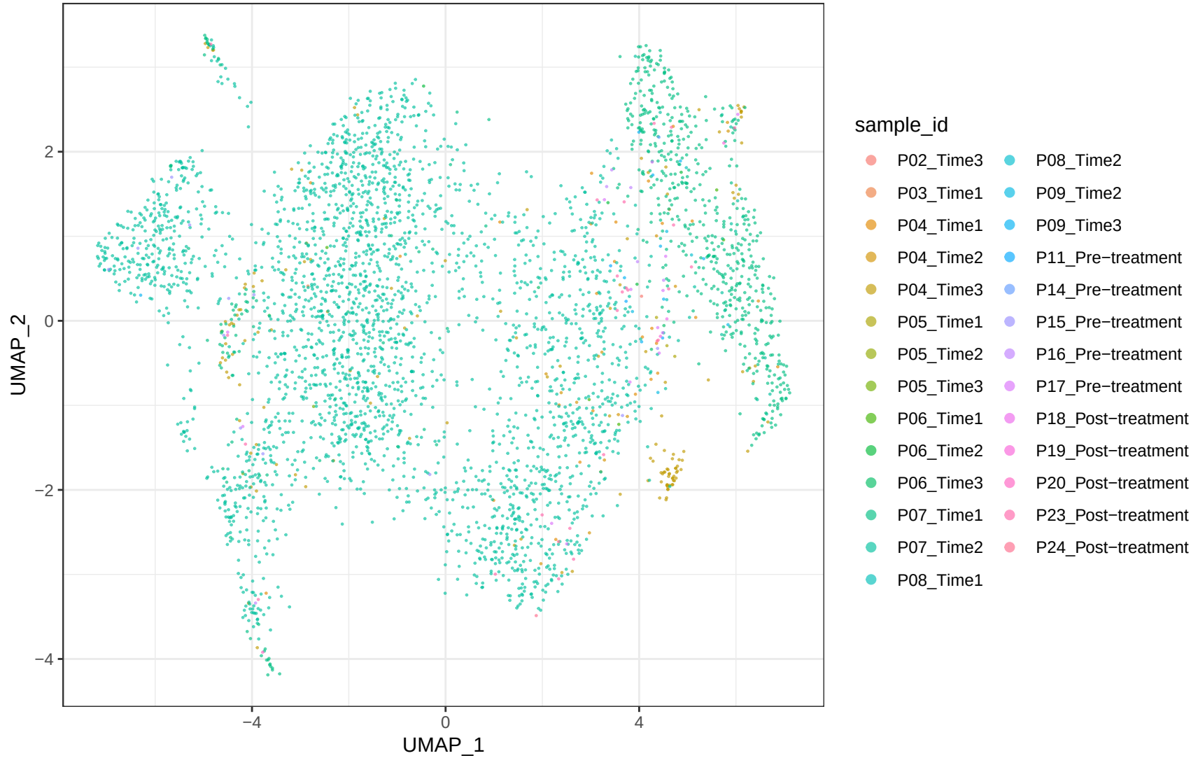
GSE158722 Myeloid_like B_harmony_patient samples
