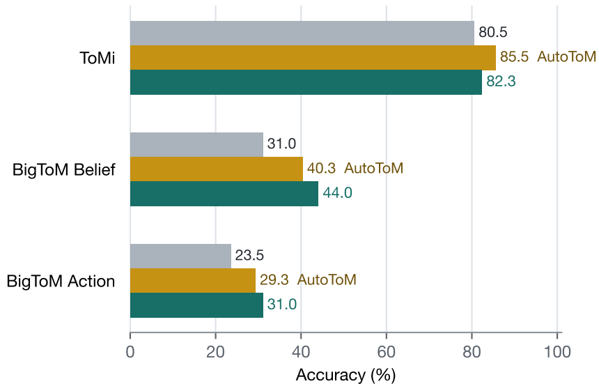
(b) Theory of Mind
