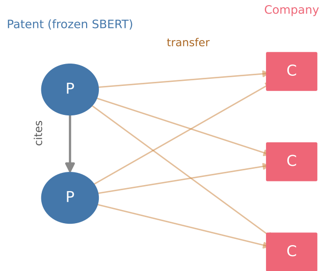
(a) Heterogeneous graph
