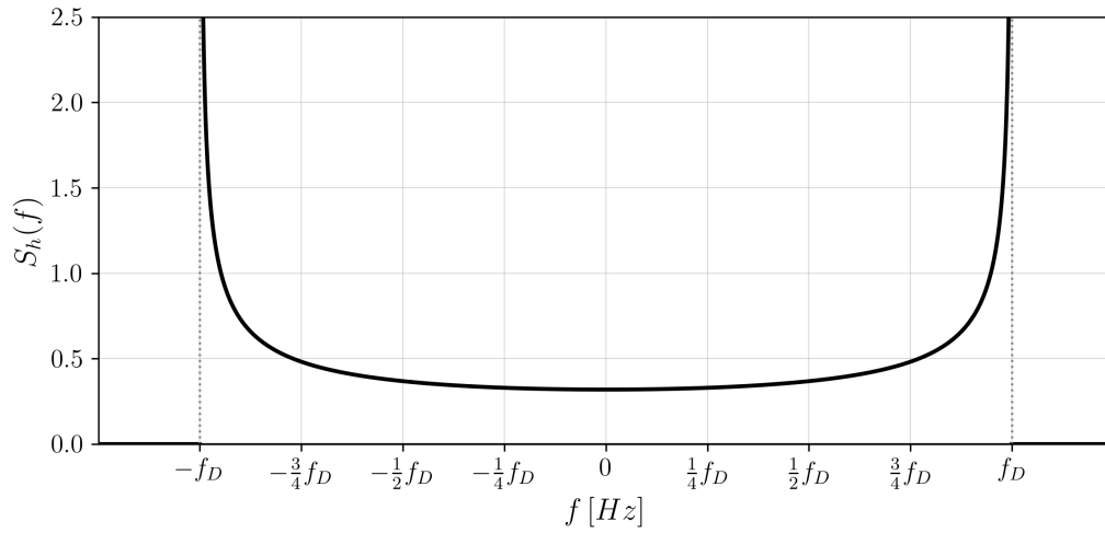
Figure C.3: The Doppler spectrum of Jakes' model.
