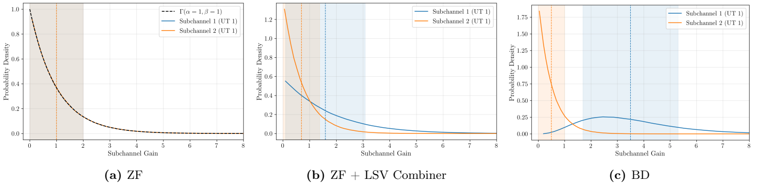
Figure 3.5: The marginal pdfs of the effective subchannel gains for a single UT in a 8 \times \{2, 2, 2, 2\} MU-MIMO system, compared between the different ZF-type precoding techniques. The expected value is indicated by a vertical dashed line, and the shaded area around the expected value corresponds to the standard deviation.
