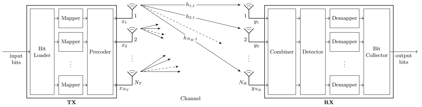
Figure 1.2: Block diagram of a SU-MIMO system.
