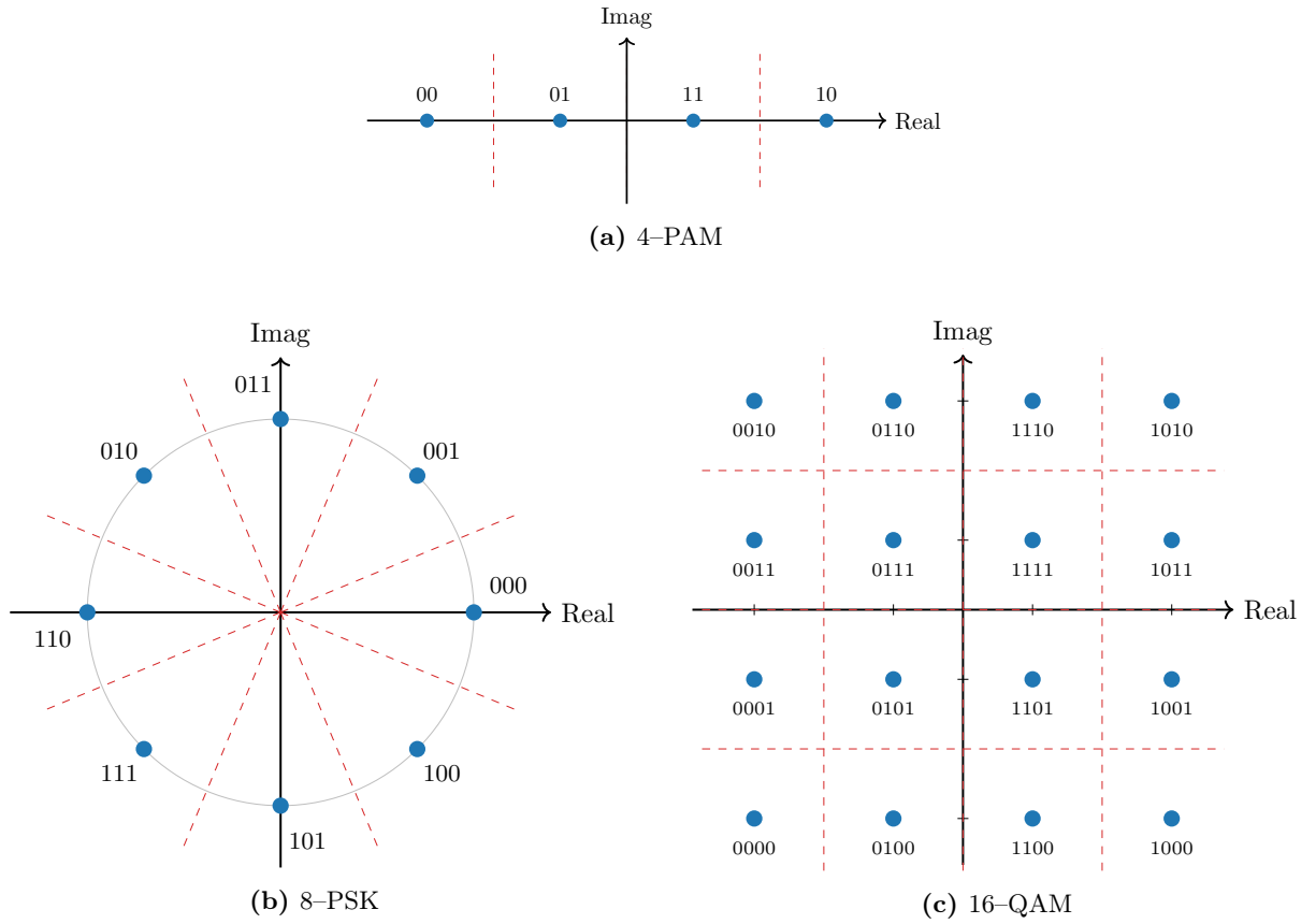
Figure B.2: An example of the constellation diagrams for different modulation schemes: 4-PAM, 8-PSK, and 16-QAM. The decision areas are bordered by the red dashed lines.
