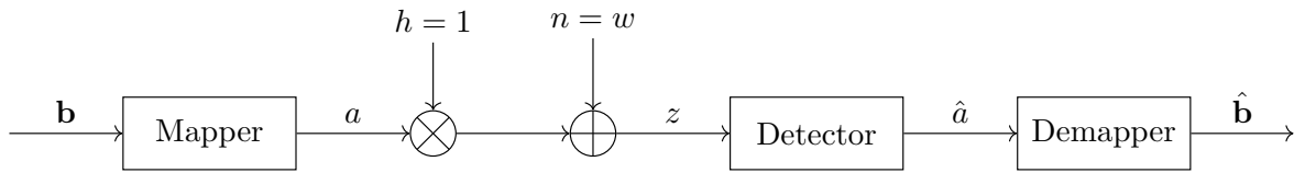
Figure B.1: Block diagram of an AWGN Channel
