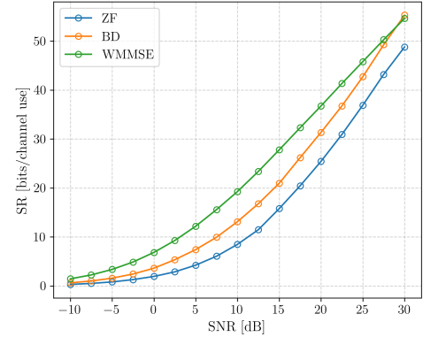
Fig. 2. Comparison of the achievable sum-rate for different precoding schemes under Rayleigh fading and perfect CSI in a 8 \times \{2, 2, 2, 2\} system.
