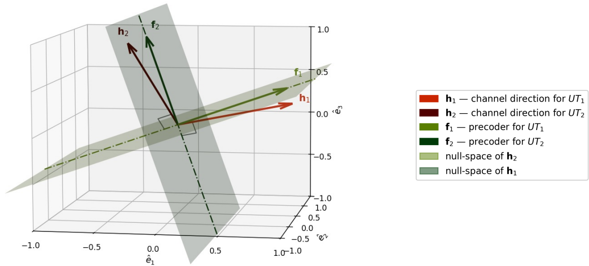
Figure 3.2: Visualization of ZF precoder for a MU-MIMO system with two single-antenna UTs and a triple-antenna BS. The channel vectors are normalized and the precoding vectors are scaled such that the effective channel gain for each data stream is equal to 1. With three transmit antennas, the null space orthogonal to each user's channel direction is two-dimensional. The ZF precoding vector is chosen as the projection of the intended user's channel direction onto this plane, which minimizes the deviation from the desired channel direction while preserving the zero-forcing constraint.
