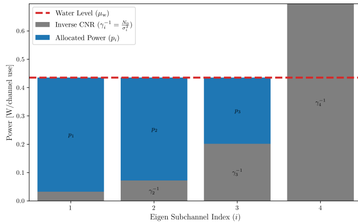
Figure 2.2: Optimal power allocation for a SU-MIMO system with 4 transmit and 4 receive antennas and a total transmit power P_T of 1 W per channel use. The system operates at an signal-to-noise ratio (SNR) of 5 dB.
