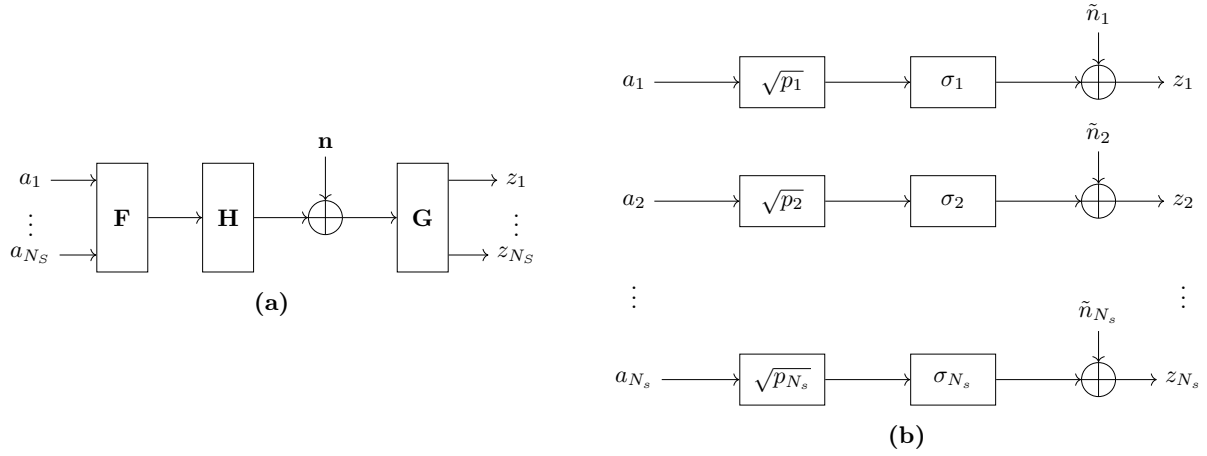
Figure 2.1: A block diagram of the original SU-MIMO channel (a) and its decomposition into parallel SISO Gaussian eigen subchannels (b) by means of the optimal precoder and combiner.
