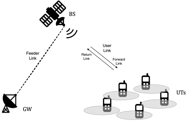
Fig. 1. Illustration of the considered system architecture for mobile satellite communications.
