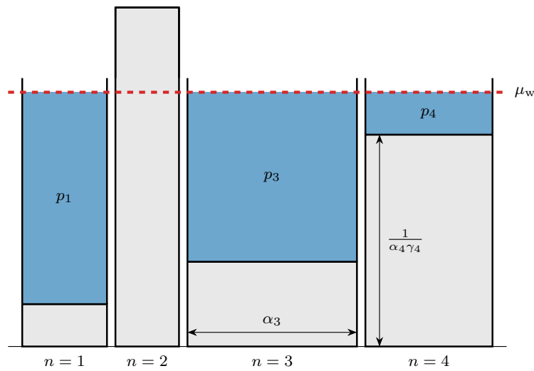
Figure A.1: A visualization of the waterfilling algorithm as the optimal power allocation strategy in a system with N = 4 channels.
