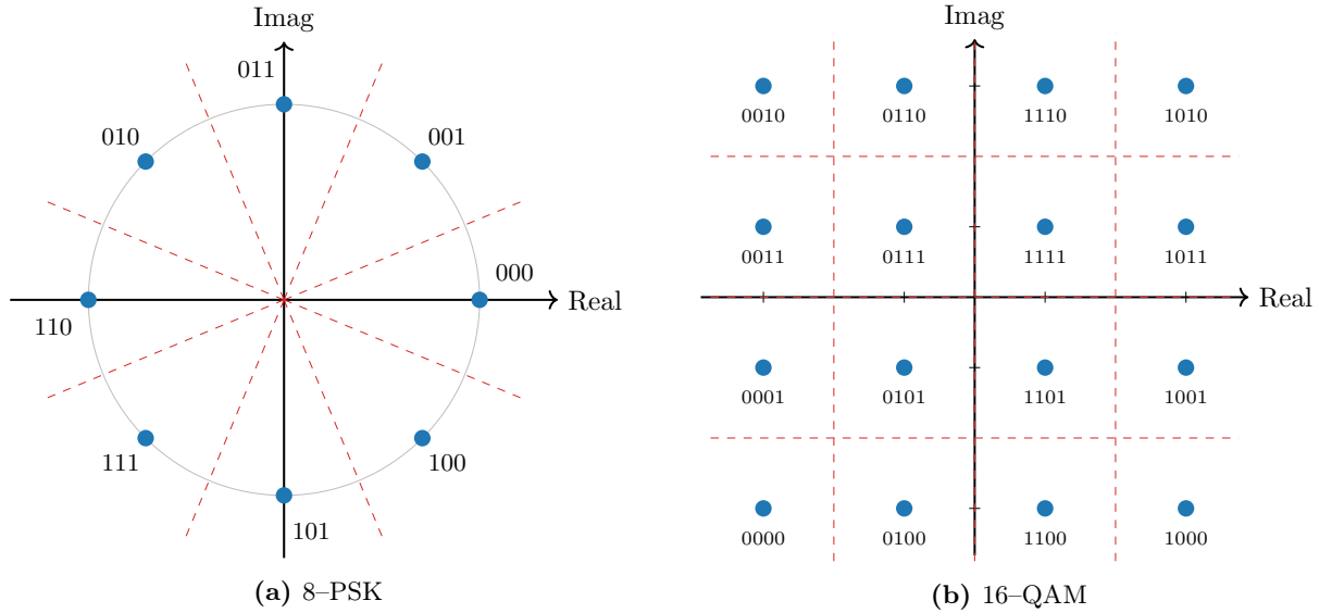
Figure B.2: An example of the constellation diagrams for two different modulation schemes: 8-PSK and 16-QAM. The decision areas are bordered by the red dashed lines. The labels show the binary mapping of the constellation points, based on Gray coding.
