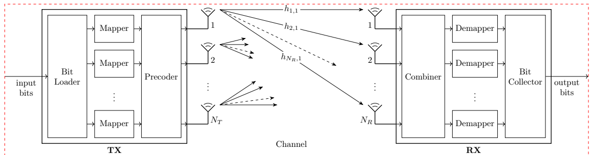
Figure 1.2: Block diagram of a SU-MIMO system.
