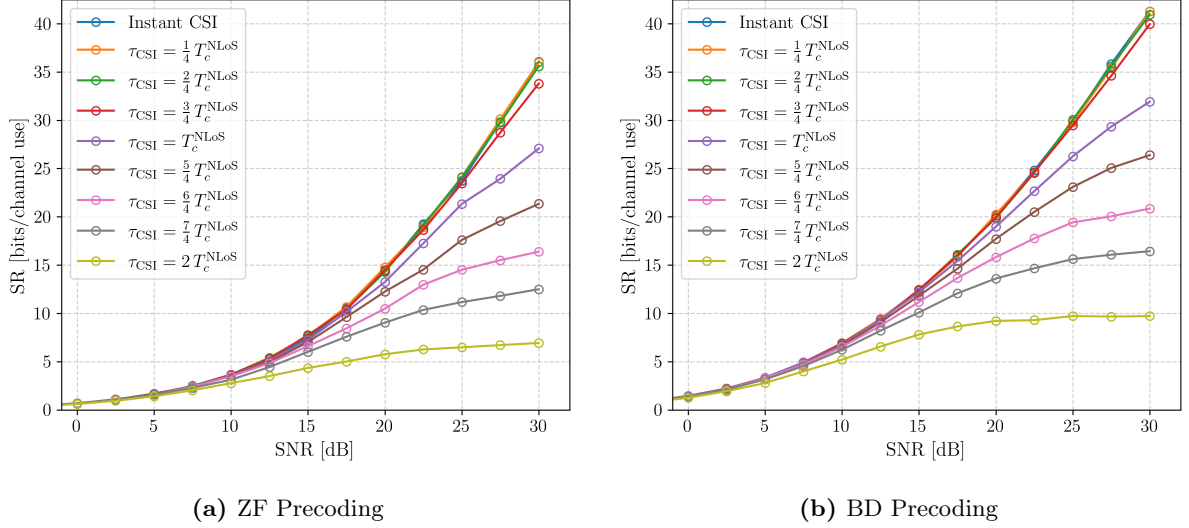
Figure 5.5: The achievable sum-rate as a function of the SNR for ZF and BD precoding with AR-based channel prediction at the UTs. The predictor uses the parameter pair selected in Section 5.3.2. The different curves correspond to different CSI feedback delays, from no delay up to a delay equal to 2 coherence periods of the NLoS component.
