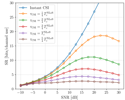
Fig. 3. Comparison of the achievable sum-rate using a WMMSE precoder for different values of the normalized CSI feedback delay.
