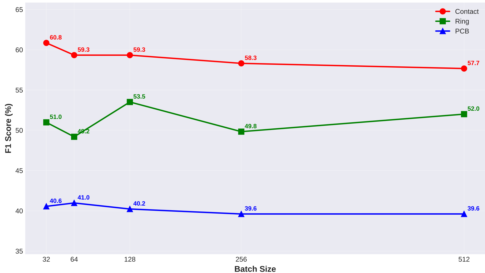
F1 Score vs Batch Size for Different Datasets
