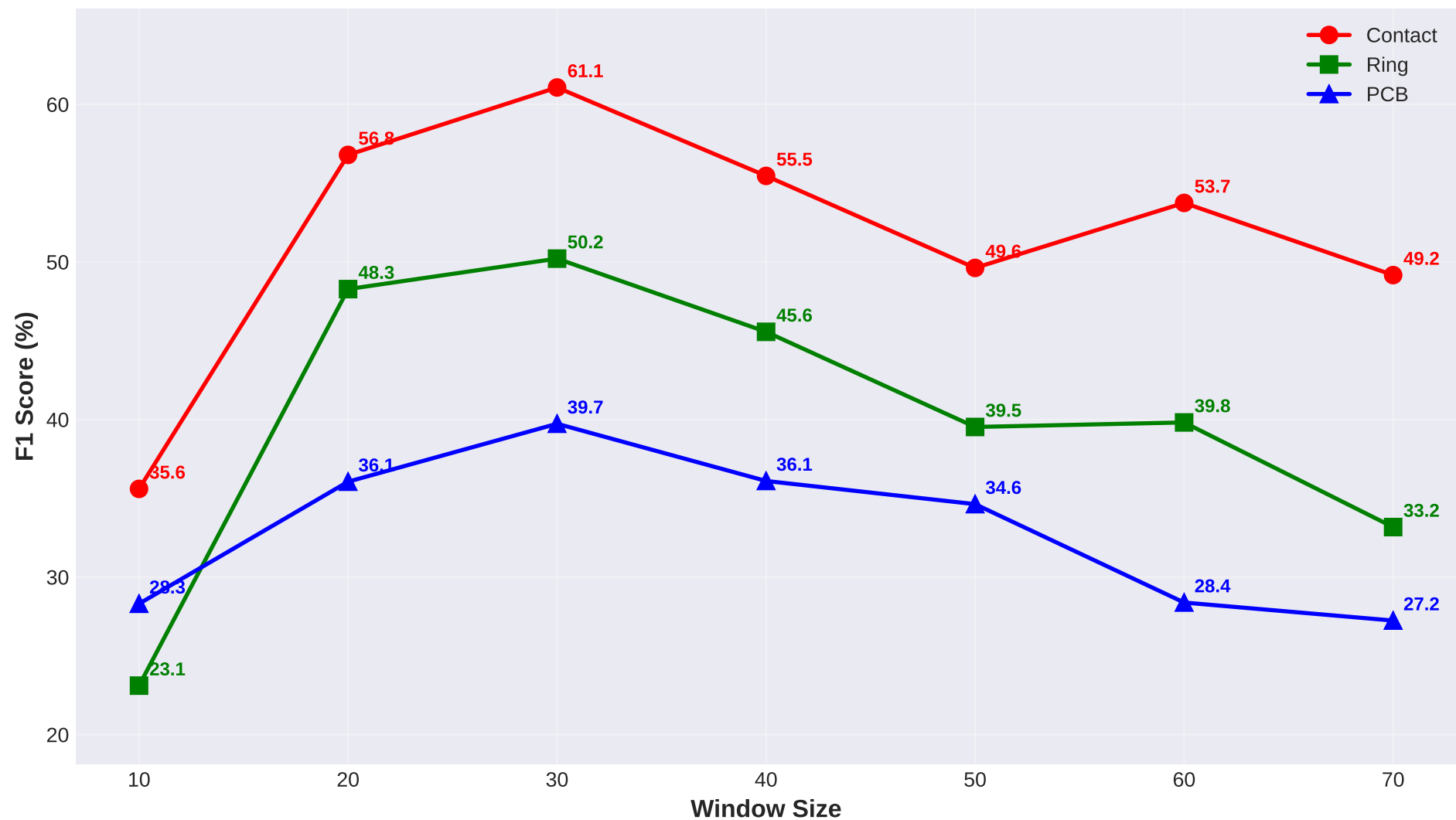
F1 Score vs Window Size for Different Datasets
