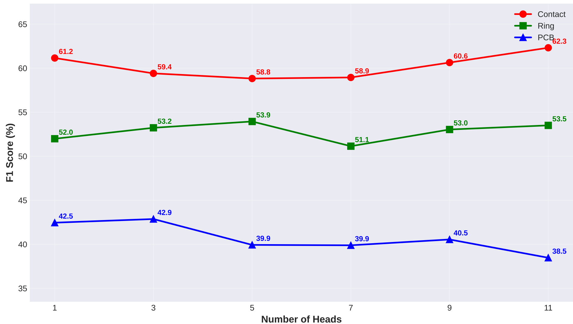
F1 Score vs Number of Heads for Different Datasets
