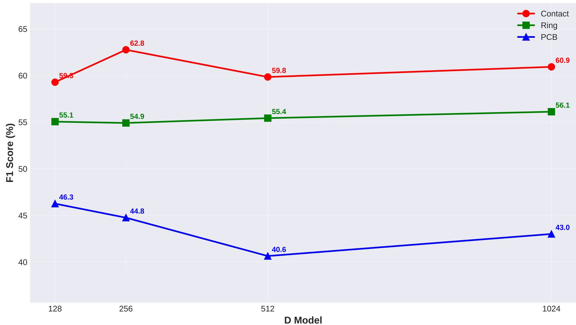
F1 Score vs D Model for Different Datasets
