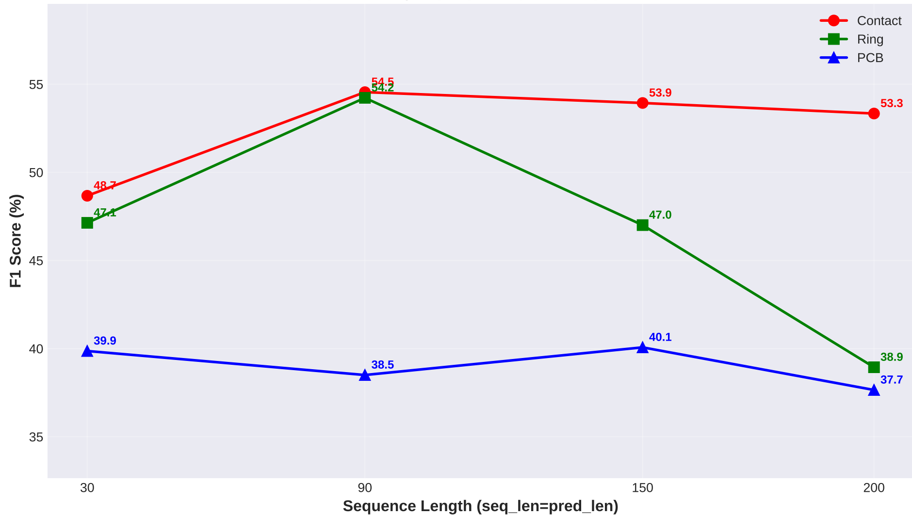
F1 Score vs Sequence Length (seq_len=pred_len) for Different Datasets
