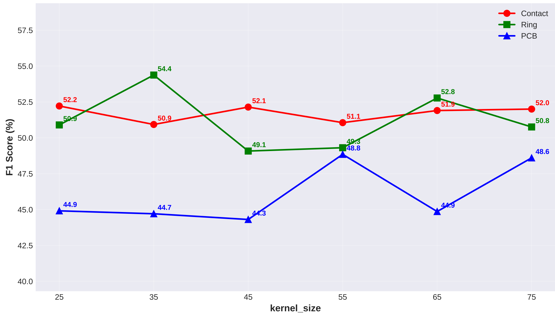
F1 Score vs kernel_size for Different Datasets
